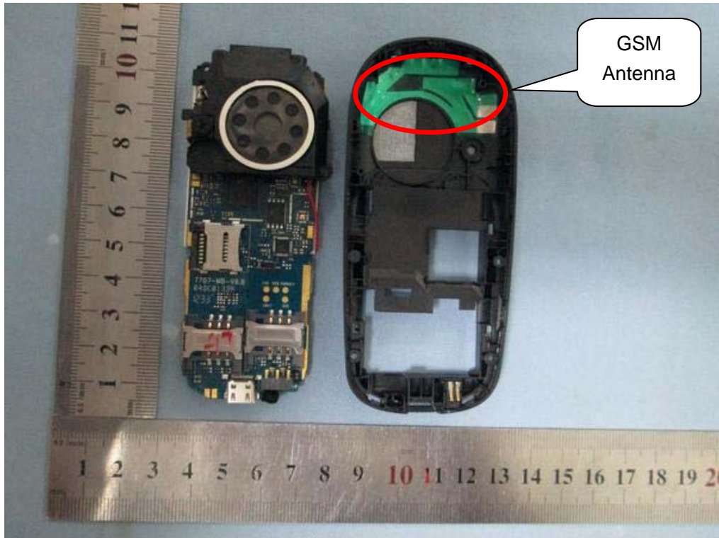
OPEN VIEW OF SAMPLE-3
