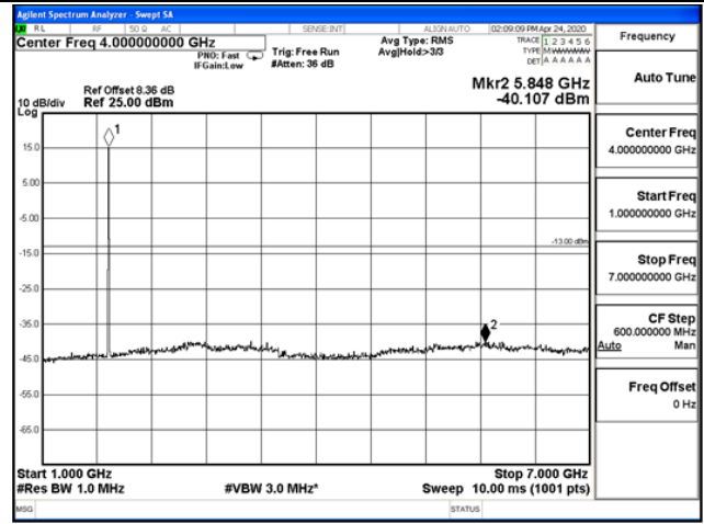
1 GHz – 7 GHz
