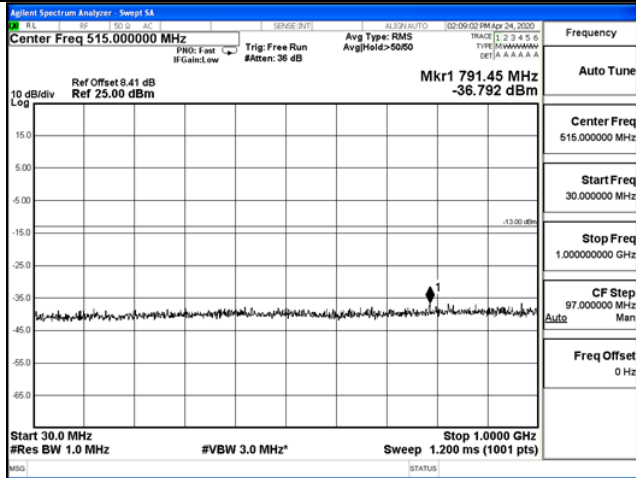
30 MHz – 1000 MHz
