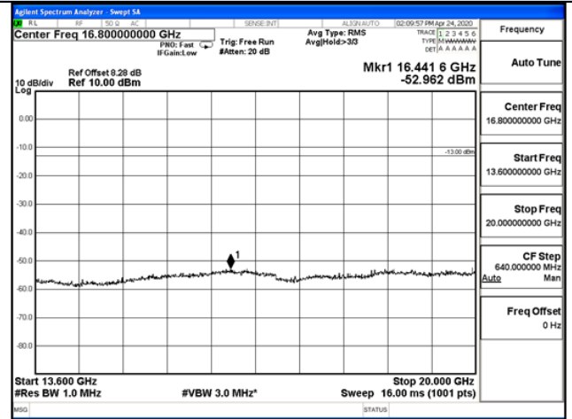
13.6 GHz – 20 GHz
