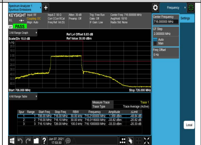
Band17-10MHz-QPSK-23780-1RB#49
