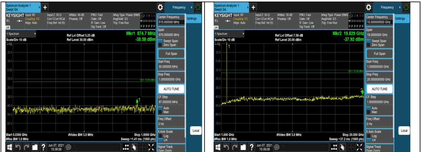
Band4-20MHz-16QAM-20050-1RB#0-Range1:30~1
