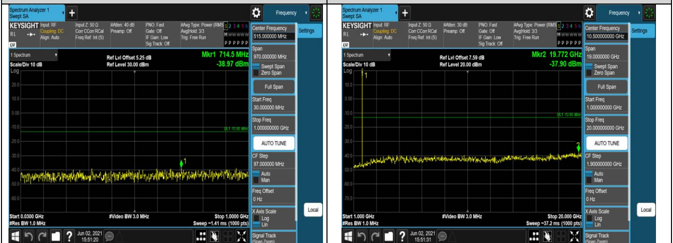
Band4-1.4MHz-16QAM-20393-1RB#0-Range1:30~1 000MHz
