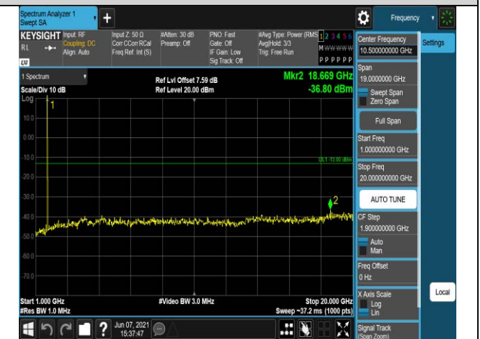
Band4-20MHz-16QAM-20175-1RB#0-Range2:1000~20
