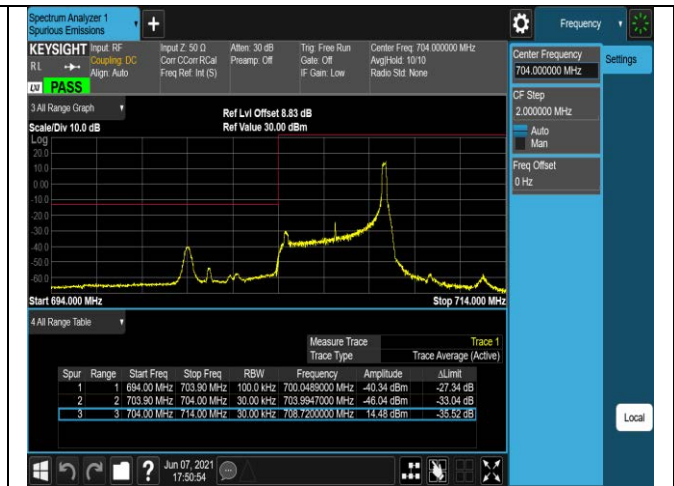
Band17-5MHz-16QAM-23825-1RB#0
