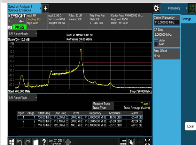
Band17-5MHz-16QAM-23755-1RB#0
