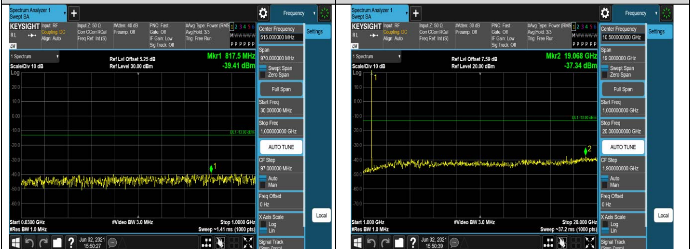
Band4-1.4MHz-16QAM-20175-1RB#0-Range1:30~1 000MHz
