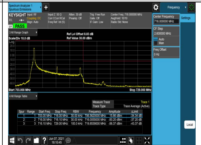
Band17-10MHz-QPSK-23800-50RB#0
