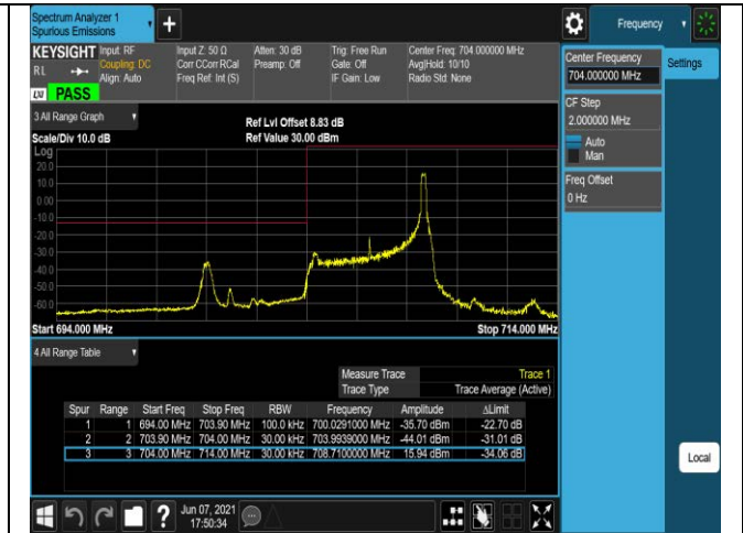
Band17-5MHz-QPSK-23825-1RB#0
