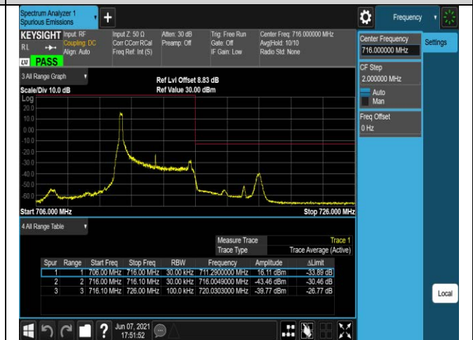
Band17-5MHz-QPSK-23825-25RB#0
