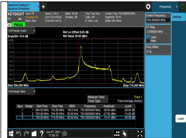
Band17-5MHz-16QAM-23755-25RB#0
