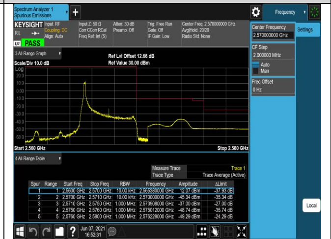
Band7-5MHz-QPSK-21425-25RB#0
