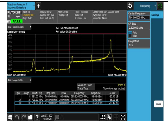
Band17-10MHz-QPSK-23800-1RB#0
