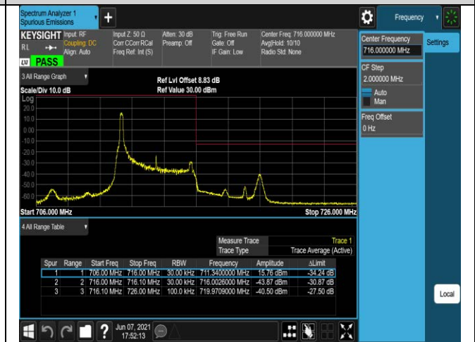
Band17-5MHz-16QAM-23825-25RB#0
