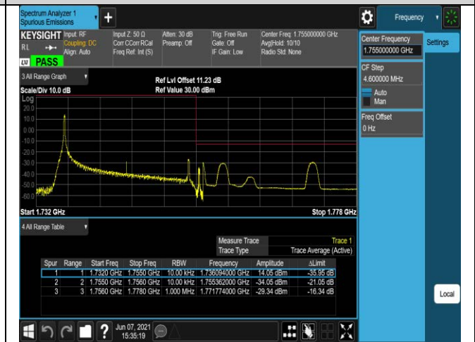
Band4-20MHz-QPSK-20300-100RB#0
