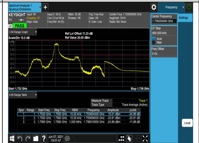
Band4-1.4MHz-QPSK-20393-6RB#0
