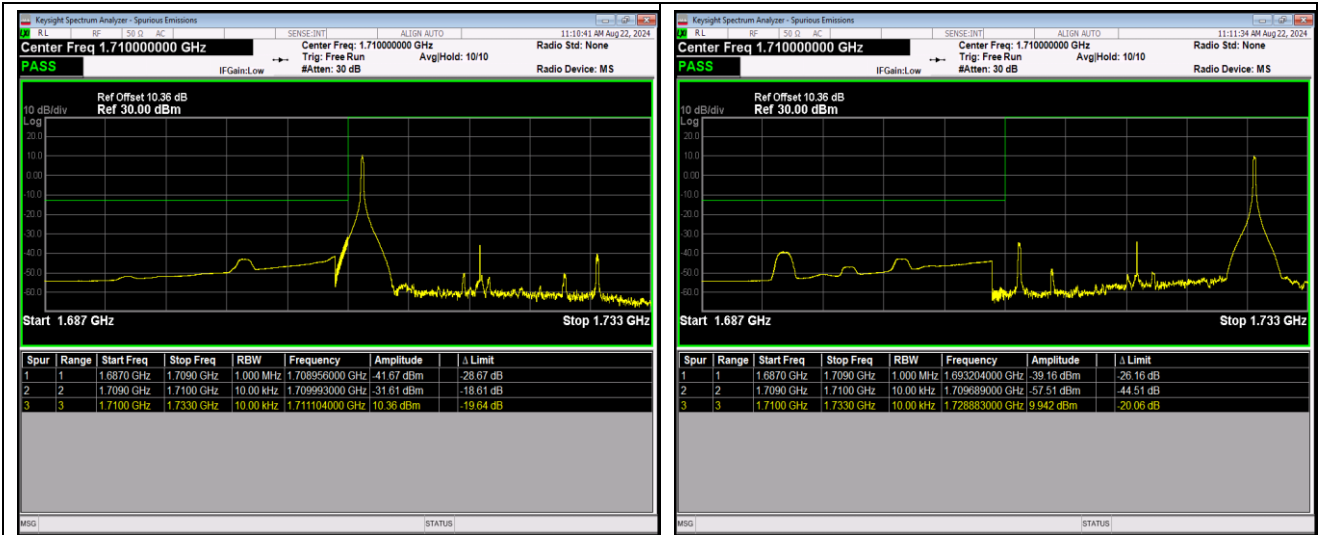
Band66-20MHz-16QAM-132072-100RB#0
