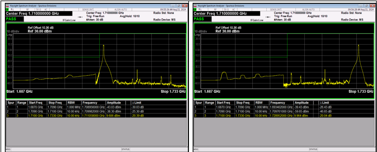
Band4-20MHz-16QAM-20050-100RB#0
