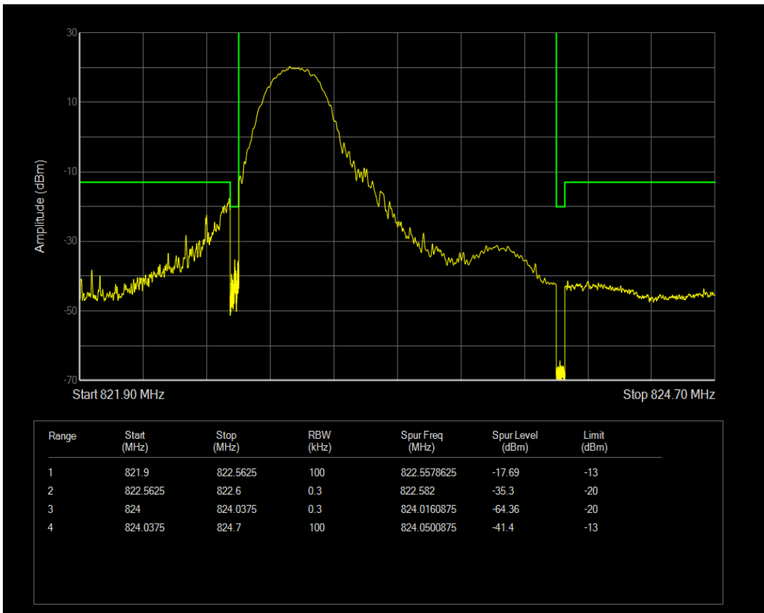
Band26(814-824) 16QAM BW=1.4MHz Channel=26783 RB Size=1 Position=#Max
