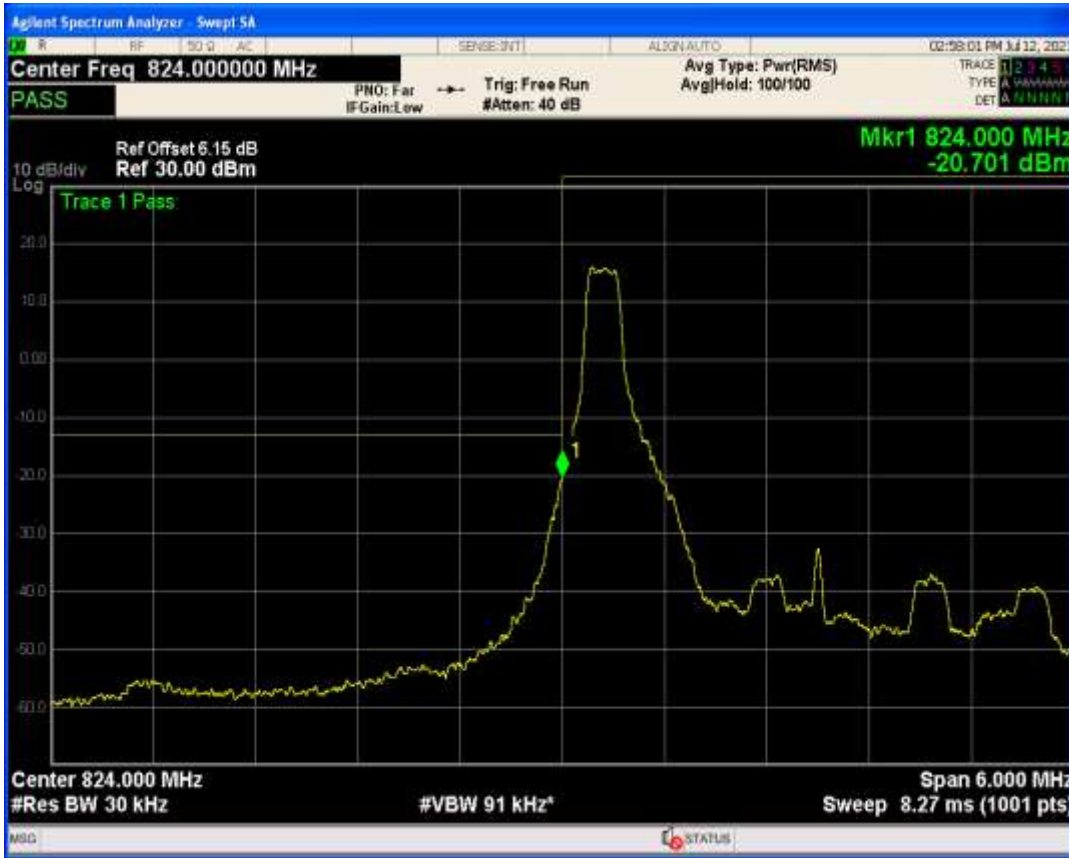
Band26b QPSK BW=3MHz Channel=26805 RB Size=1 Position=#Max
