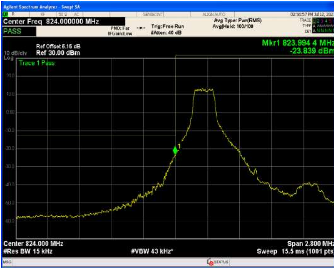
Band26b QPSK BW=1.4MHz Channel=26797 RB Size=1 Position=#Max
