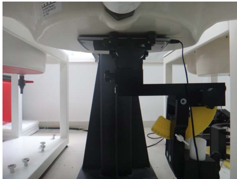
0mm Body-worn Rear Side with Headset Setup Photo
