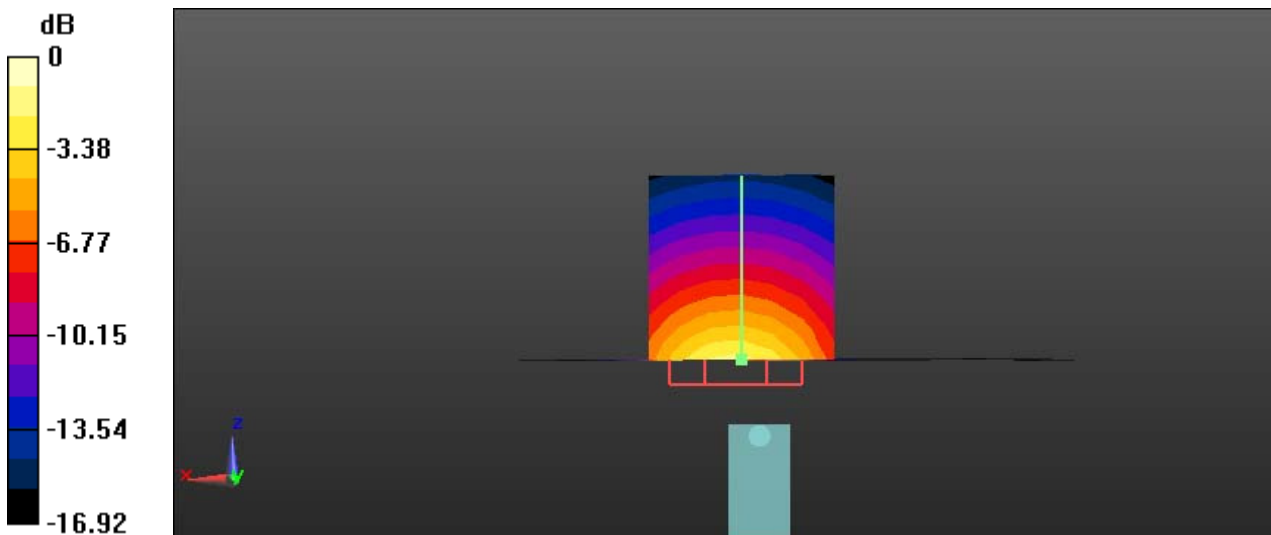
0 dB = 39.4 W/kg = 15.95 dBW/kg
