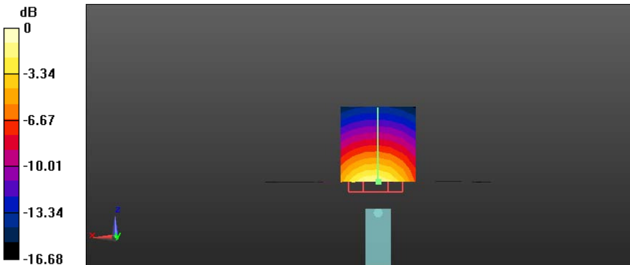
0 dB = 41.9 W/kg = 16.22 dBW/kg
