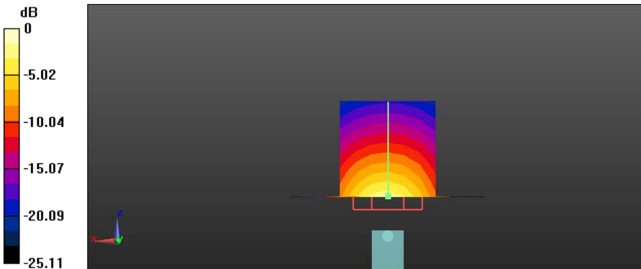
0 dB = 67.6 W/kg = 18.30 dBW/kg
