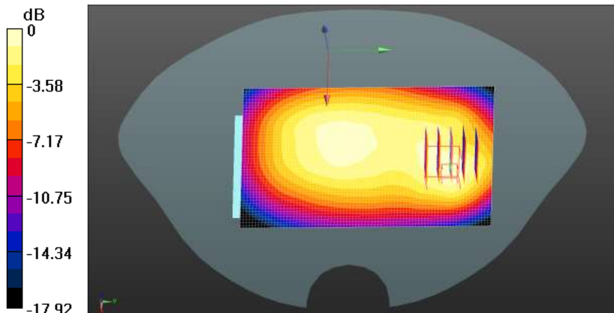
0 dB = 0.292 W/kg = -5.35 dBW/kg
