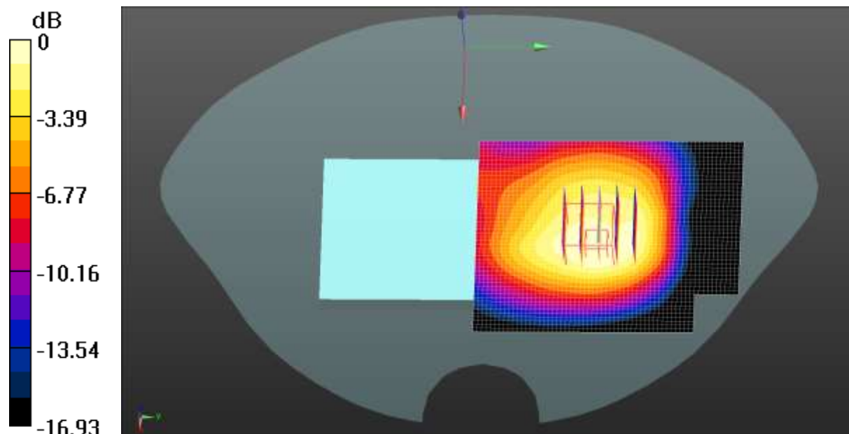
0 dB = 0.704 W/kg = -1.52 dBW/kg
