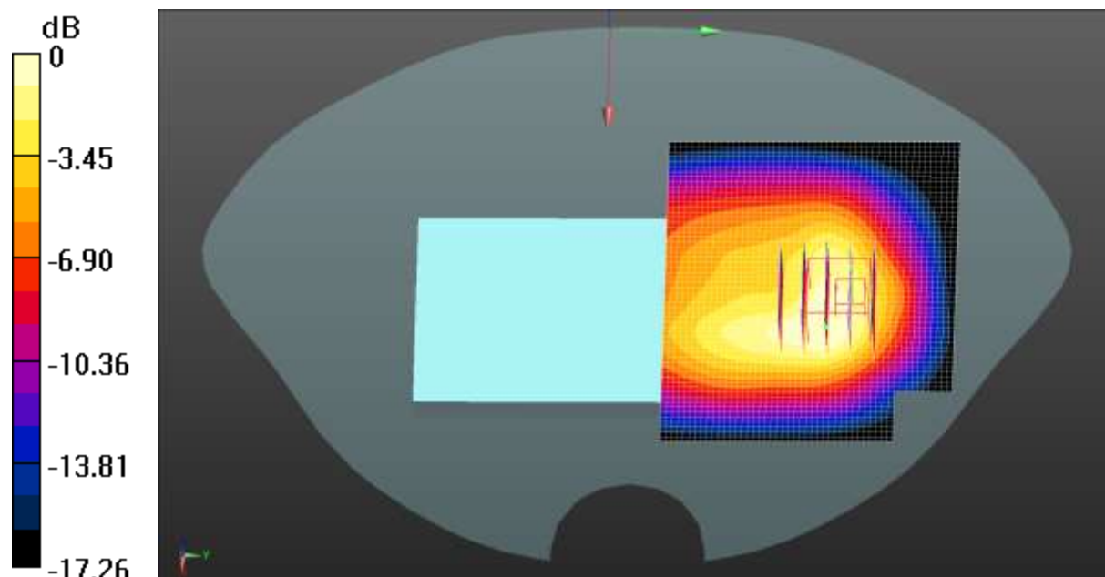
0 dB = 0.900 W/kg = -0.46 dBW/kg
