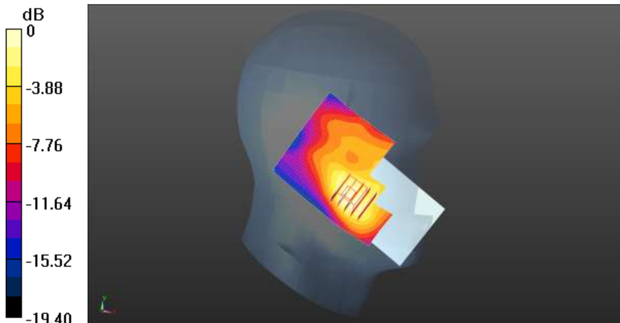
0 dB = 0.289 W/kg = -5.39 dBW/kg
