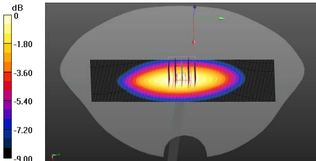
0 dB = 0.948 W/kg = -0.23 dBW/kg
