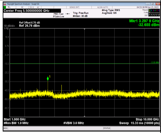
Band5-1.4MHz-QPSK-20407-1RB#0-Range2:1000~10000MHz
