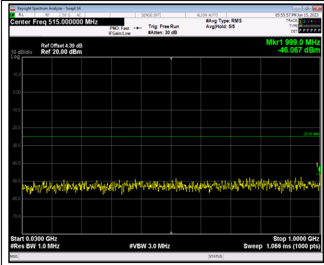
Band7-20MHz-QPSK-21350-1RB#0-Range1:30~100 OMHz
