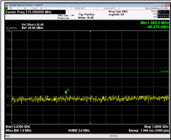
Band7-5MHz-QPSK-21425-1RB#0-Range1:30~1000 MHz
