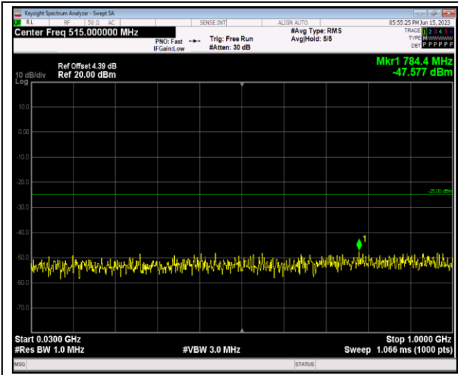
Band7-20MHz-QPSK-21100-1RB#0-Range1:30~100 OMHz
