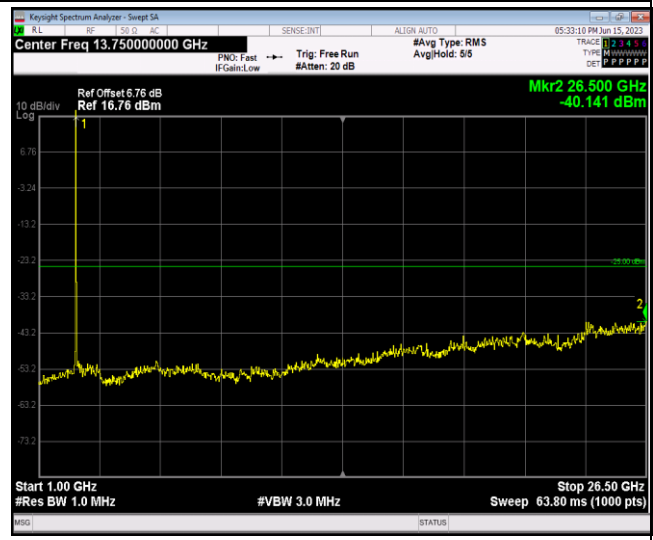
Band7-5MHz-16QAM-20775-1RB#0-Range2:1000~26500MHz
