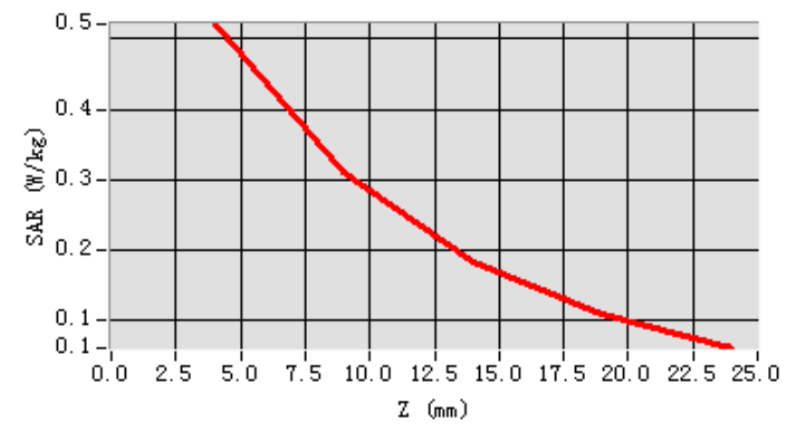
SAR, Z Axis Scan (X = 12, Y = -14)
