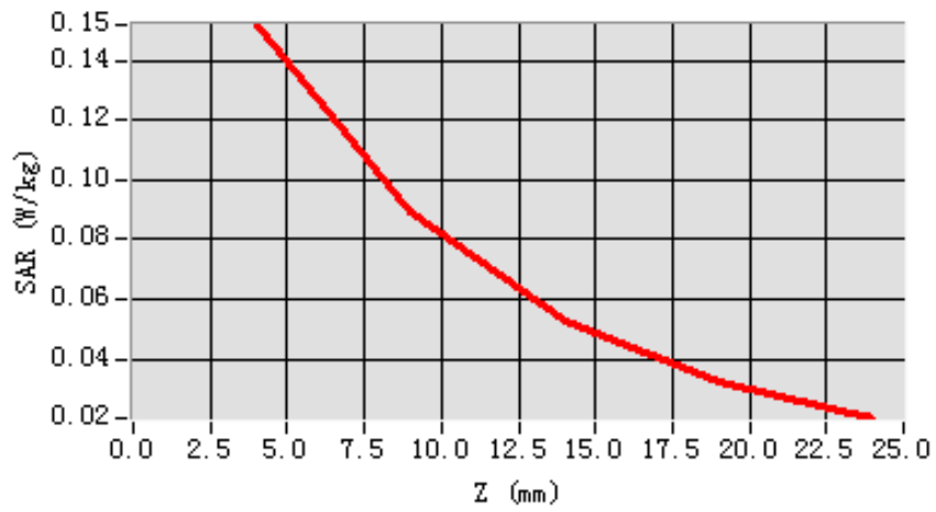
SAR, Z Axis Scan (X = -20, Y = 27)
