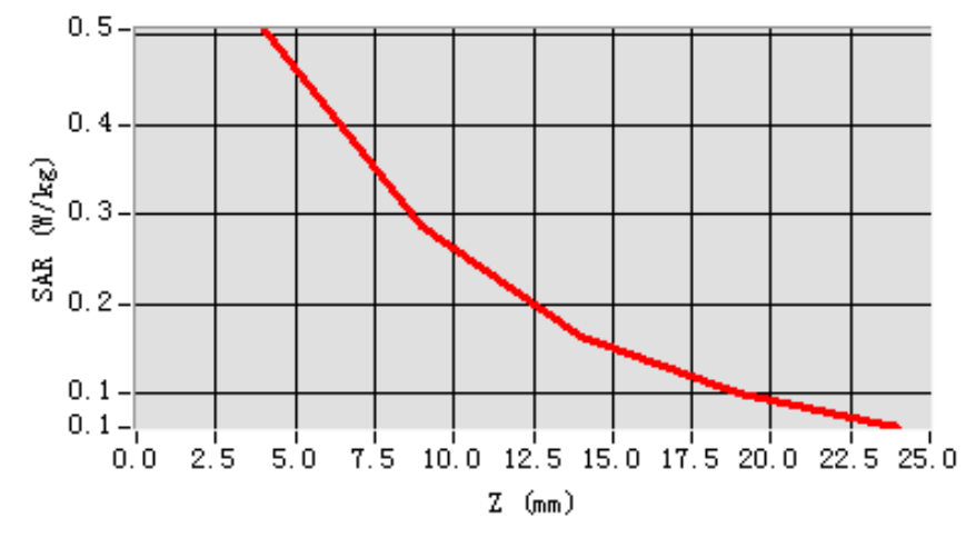
SAR, Z Axis Scan (X = 18, Y = -13)
