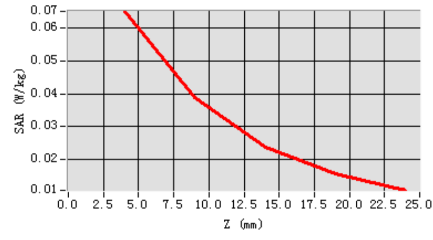
SAR, Z Axis Scan (X = 1, Y = 25)
