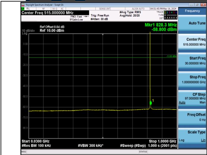
Band5_1.4MHz_QPSK_20407_1RB#0_30~1000_30~1000
