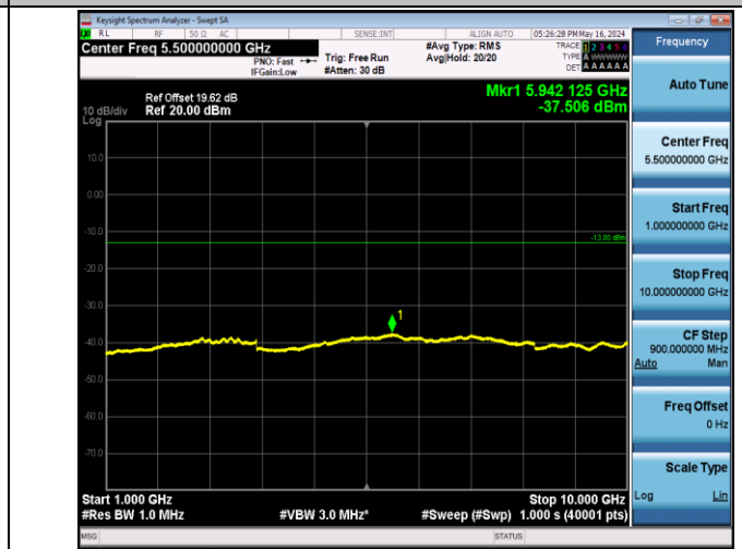
Band5_10MHz_16QAM_20525_1RB#0_1000~10000_1000~1000
