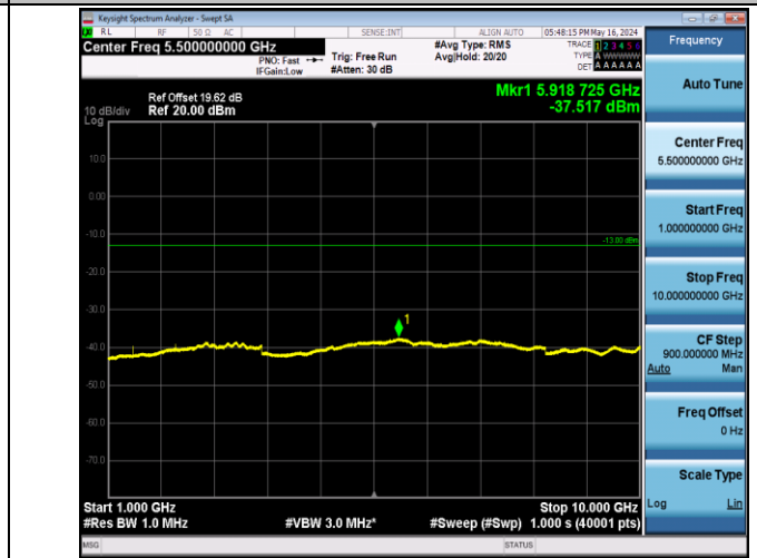
Band12_1.4MHz_16QAM_23173_1RB#0_1000~10000_1000~1000 00
