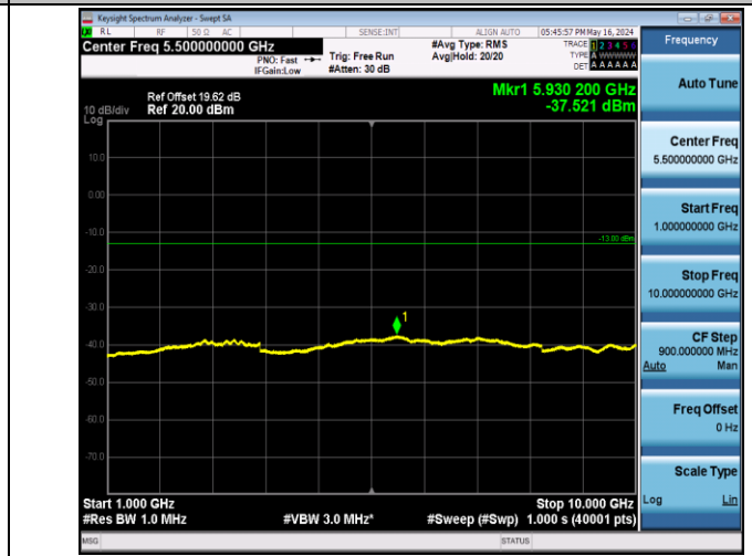
Band12_1.4MHz_16QAM_23095_1RB#0_1000~10000_1000~1000 00
