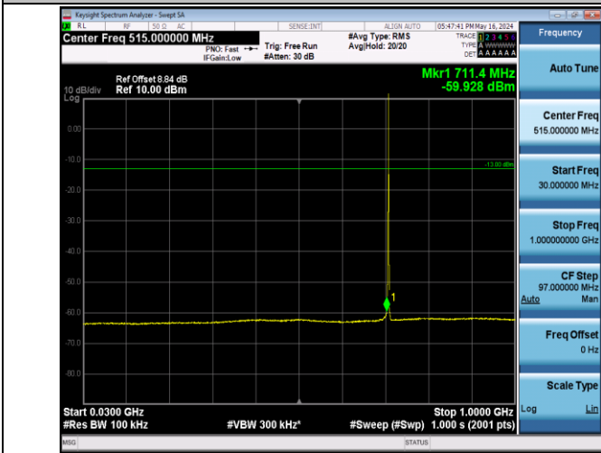
Band12_1.4MHz_16QAM_23173_1RB#0_30~1000_30~1000
