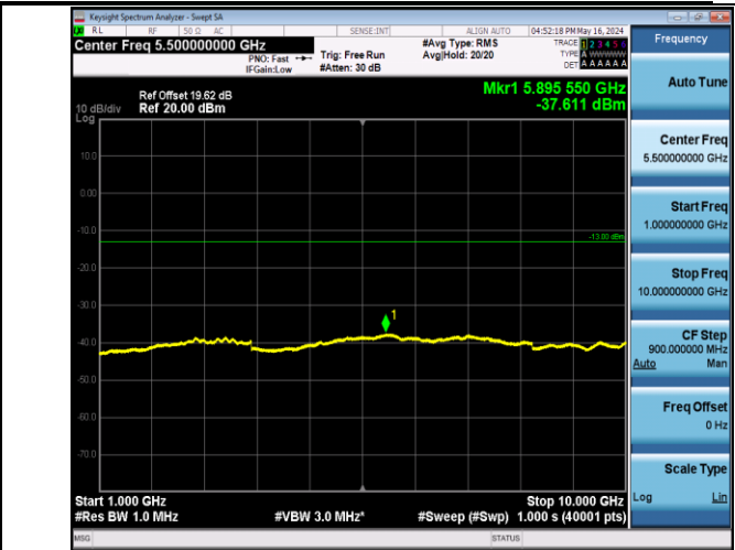
Band5_1.4MHz_QPSK_20407_1RB#0_1000~10000_1000~10000
