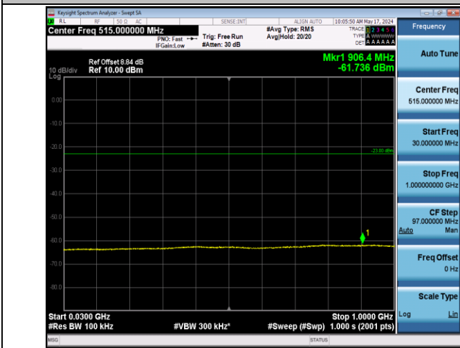
Band66_1.4MHz_QPSK_132322_1RB#0_30~1000_30~1000
