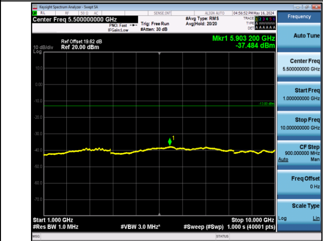
Band5_1.4MHz_QPSK_20643_1RB#0_1000~10000_1000~10000
