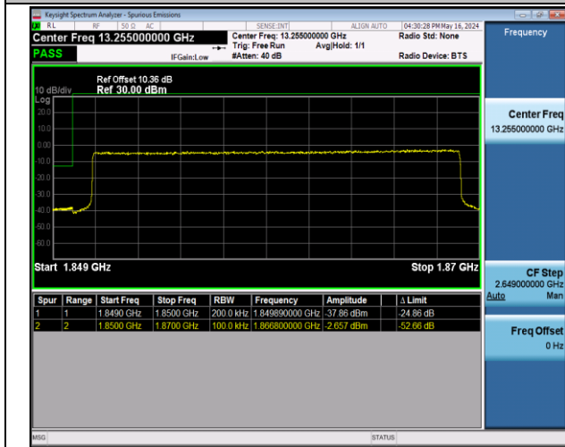
Band2_20MHz_16QAM_18700_100RB#0
