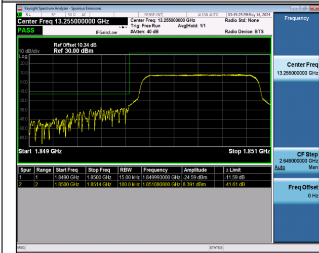
Band2_1.4MHz_16QAM_18607_6RB#0
