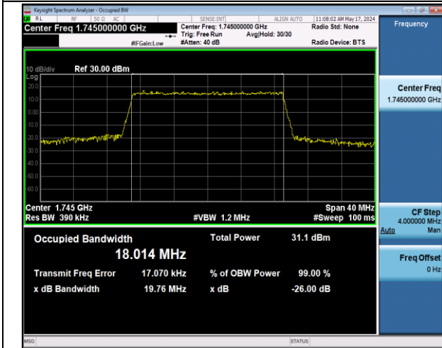
Band66-20MHz-16QAM-132322-100RB#0-PASS
