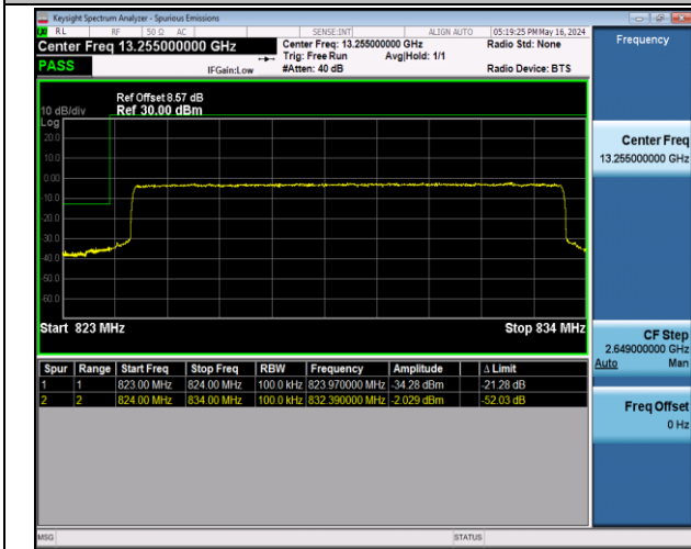
Band5_10MHz_16QAM_20450_50RB#0
