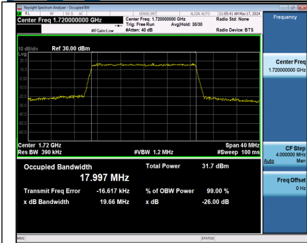
Band66-20MHz-QPSK-132072-100RB#0-PASS
