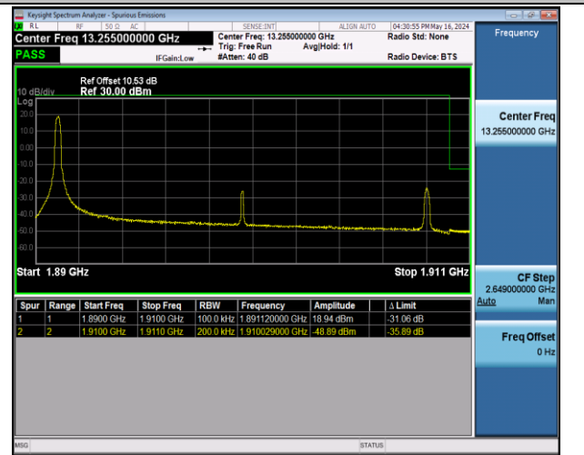
Band2_20MHz_16QAM_19100_1RB#0
