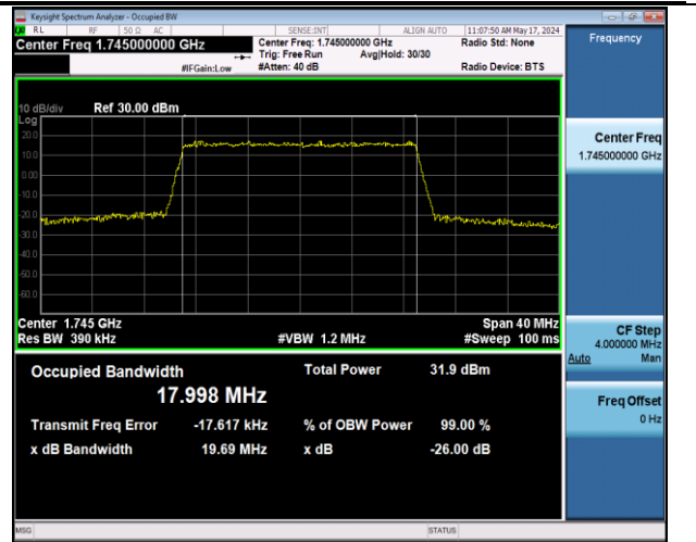
Band66-20MHz-QPSK-132322-100RB#0-PASS
