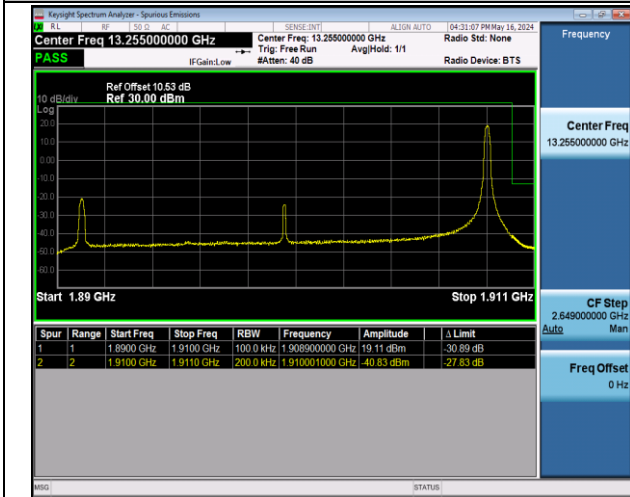
Band2_20MHz_QPSK_19100_1RB#99
