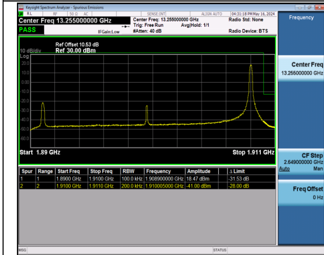
Band2_20MHz_16QAM_19100_1RB#99
