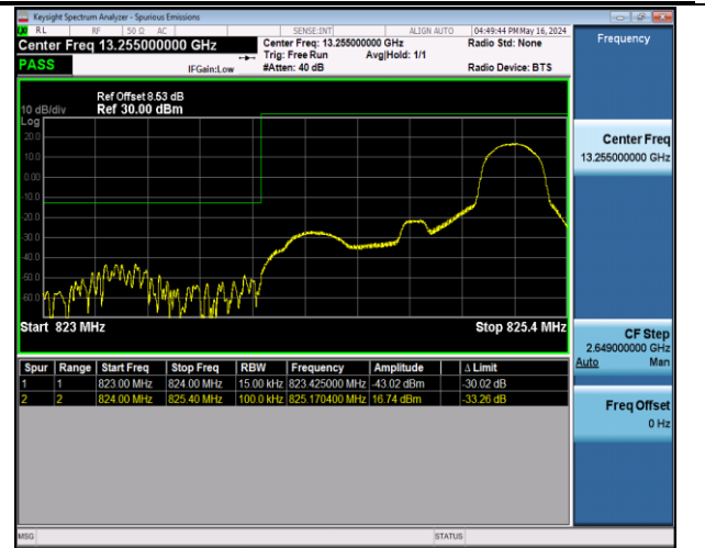
Band5_1.4MHz_16QAM_20407_1RB#5
