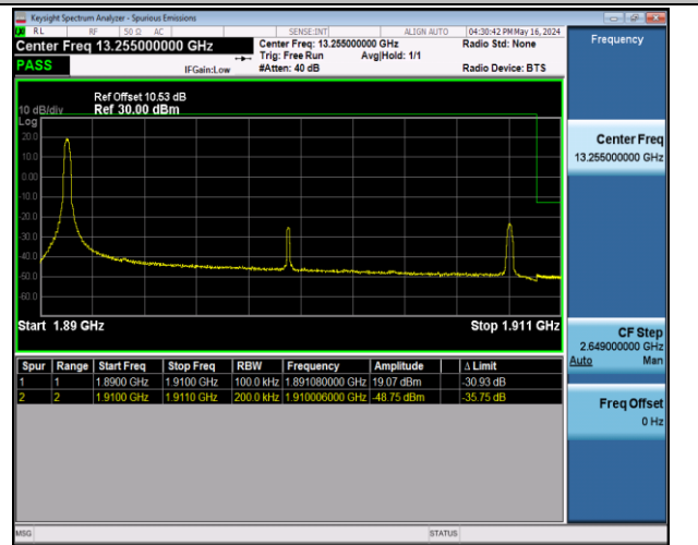
Band2_20MHz_QPSK_19100_1RB#0
