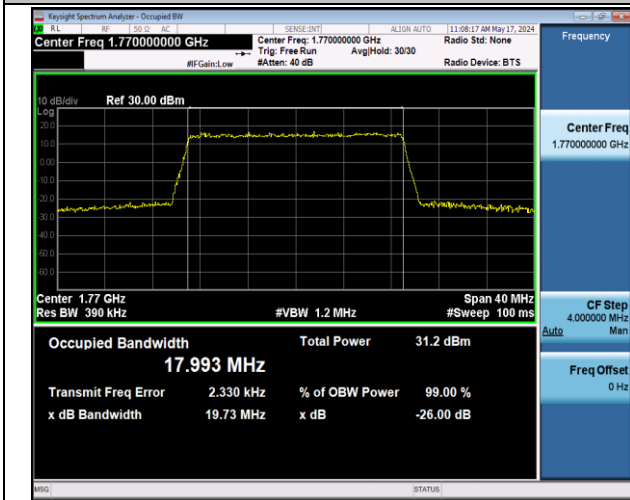
Band66-20MHz-QPSK-132572-100RB#0-PASS
