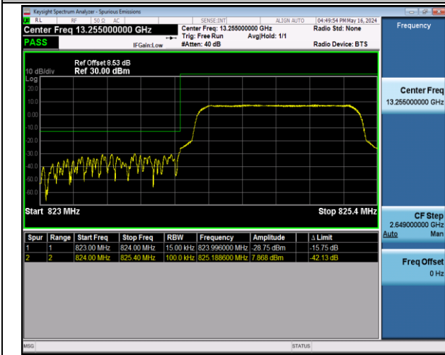
Band5_1.4MHz_QPSK_20407_6RB#0
