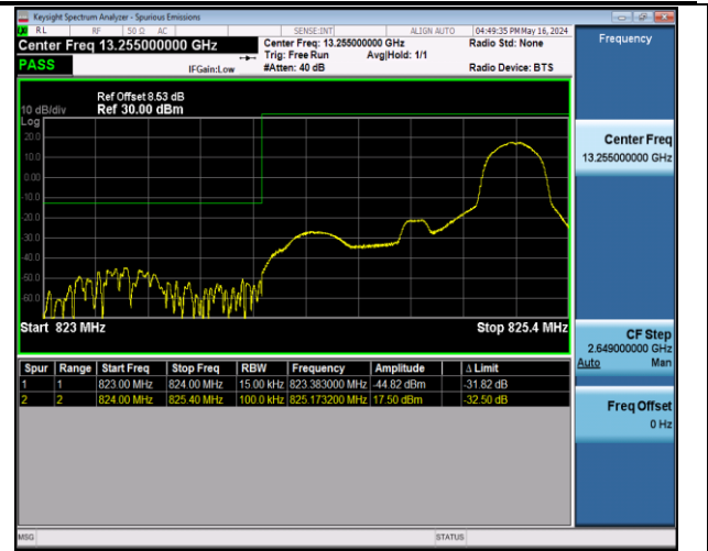
Band5_1.4MHz_QPSK_20407_1RB#5
