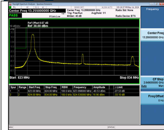
Band5_10MHz_16QAM_20450_1RB#0
