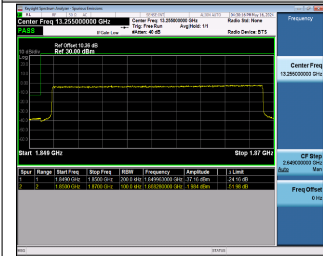
Band2_20MHz_QPSK_18700_100RB#0
