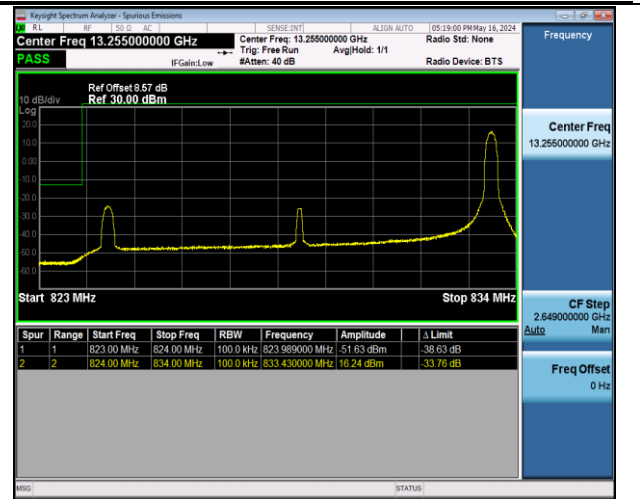
Band5_10MHz_16QAM_20450_1RB#49
