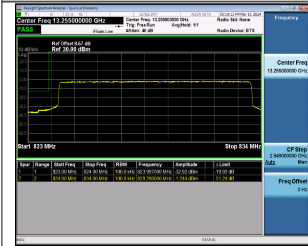
Band5_10MHz_QPSK_20450_50RB#0
