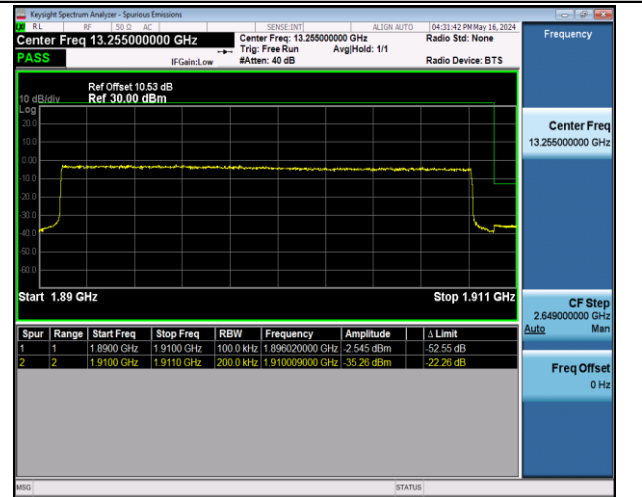
Band2_20MHz_16QAM_19100_100RB#0
