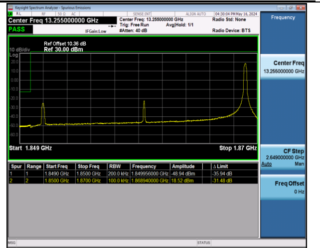
Band2_20MHz_16QAM_18700_1RB#99
