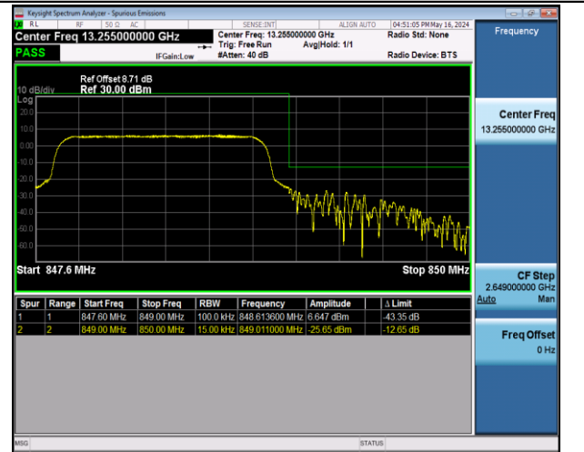
Band5_1.4MHz_16QAM_20643_6RB#0
