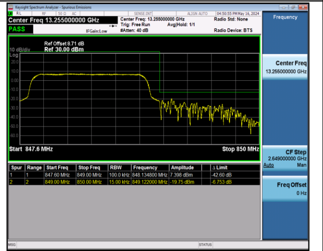
Band5_1.4MHz_QPSK_20643_6RB#0
