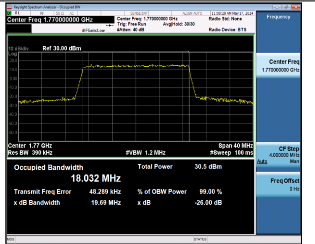
Band66-20MHz-16QAM-132572-100RB#0-PASS
