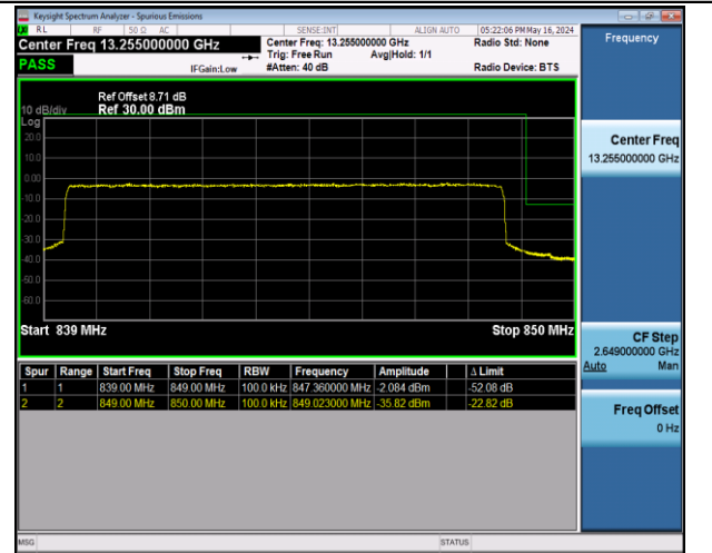
Band5_10MHz_16QAM_20600_50RB#0
