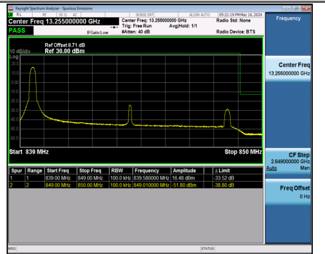
Band5_10MHz_16QAM_20600_1RB#0
