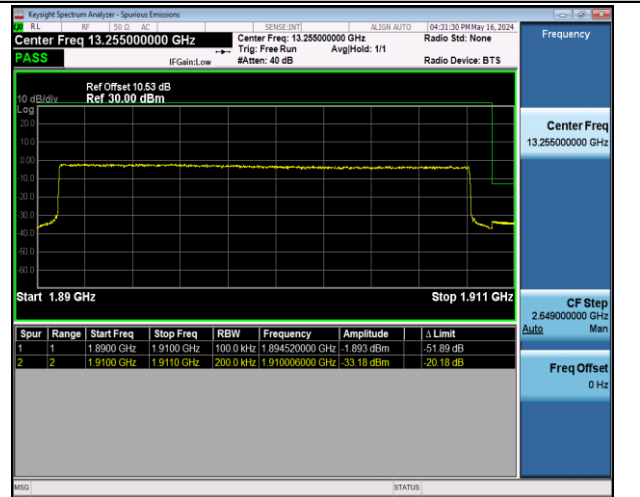
Band2_20MHz_QPSK_19100_100RB#0
