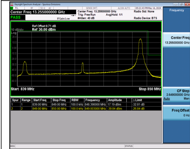
Band5_10MHz_16QAM_20600_1RB#49
