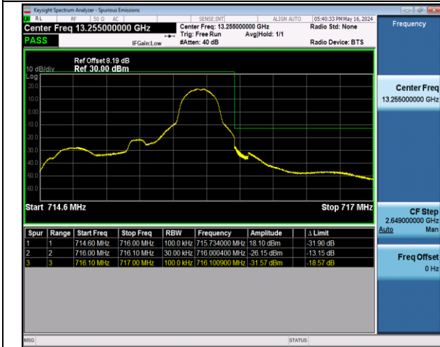
Band12_1.4MHz_QPSK_23173_1RB#5
