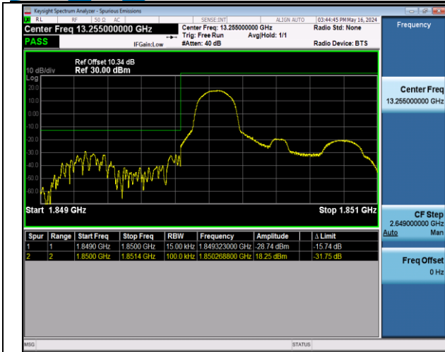
Band2_1.4MHz_16QAM_18607_1RB#0
