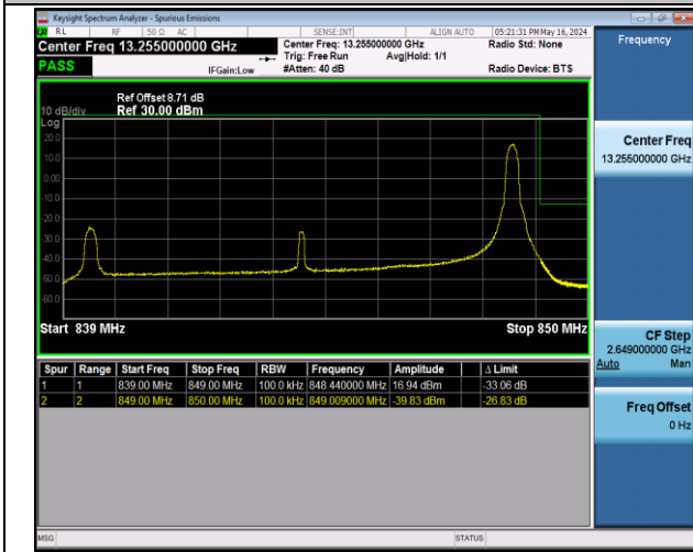
Band5_10MHz_QPSK_20600_1RB#49
