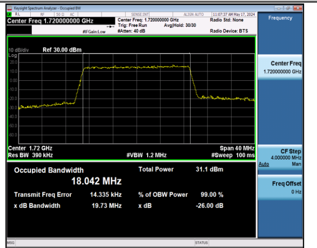
Band66-20MHz-16QAM-132072-100RB#0-PASS
