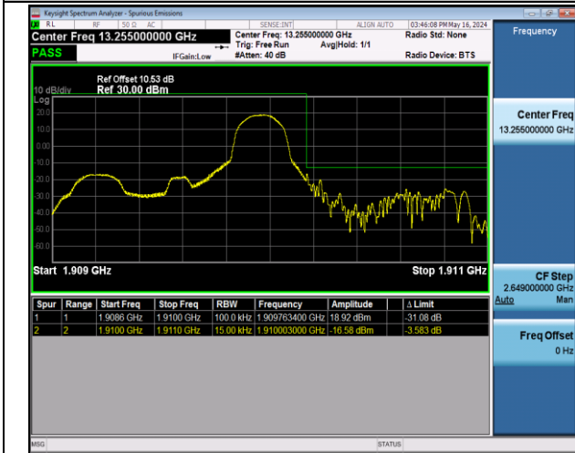
Band2_1.4MHz_16QAM_19193_1RB#5
