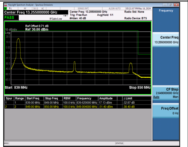
Band5_10MHz_QPSK_20600_1RB#0
