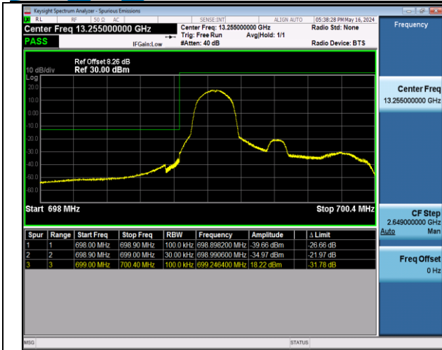
Band12_1.4MHz_QPSK_23017_1RB#0
