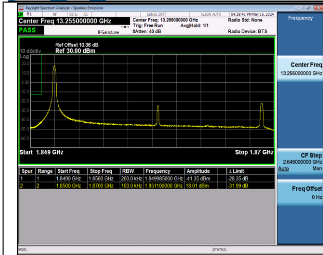
Band2_20MHz_16QAM_18700_1RB#0
