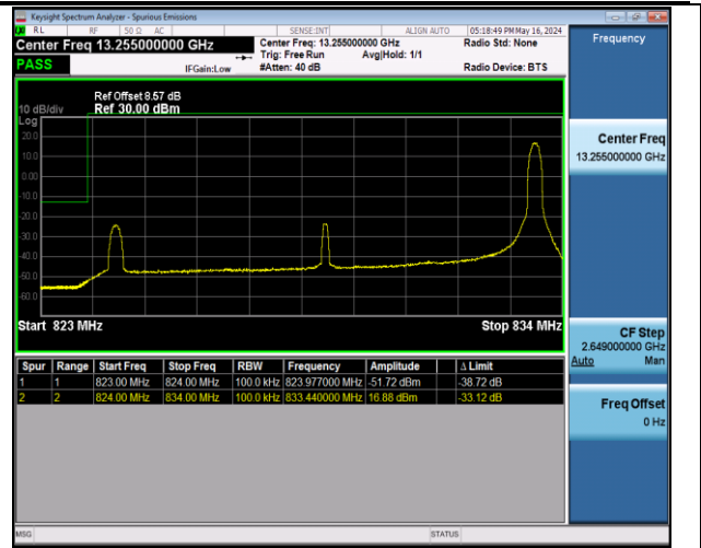
Band5_10MHz_QPSK_20450_1RB#49
