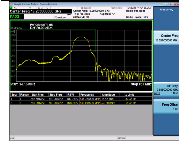
Band5_1.4MHz_16QAM_20643_1RB#5
