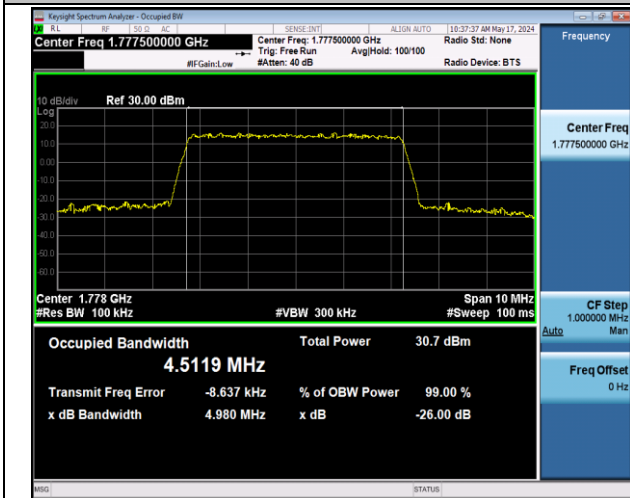
Band66-5MHz-QPSK-132647-25RB#0-PASS
