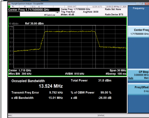
Band66-15MHz-QPSK-132047-75RB#0-PASS
