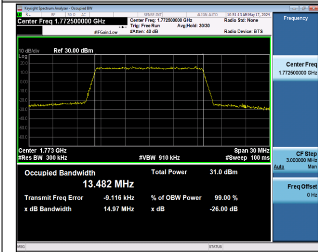
Band66-15MHz-QPSK-132597-75RB#0-PASS
