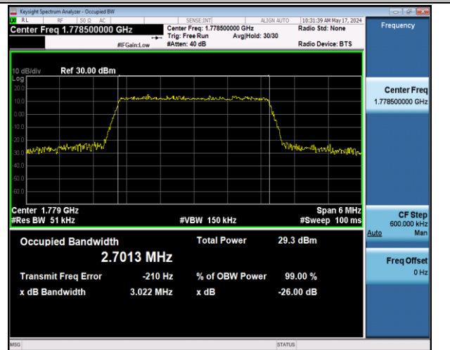
Band66-3MHz-16QAM-132657-15RB#0-PASS
