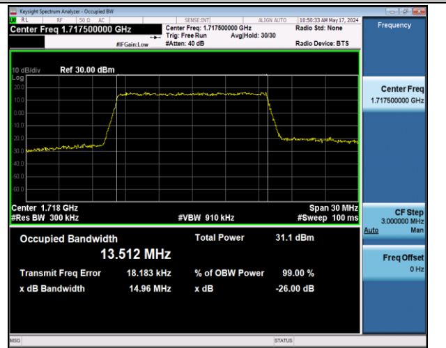
Band66-15MHz-16QAM-132047-75RB#0-PASS
