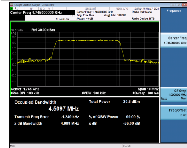
Band66-5MHz-16QAM-132322-25RB#0-PASS
