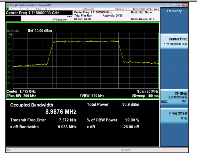
Band66-10MHz-16QAM-132022-50RB#0-PASS
