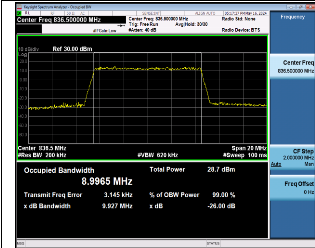
Band5-10MHz-16QAM-20525-50RB#0-PASS
