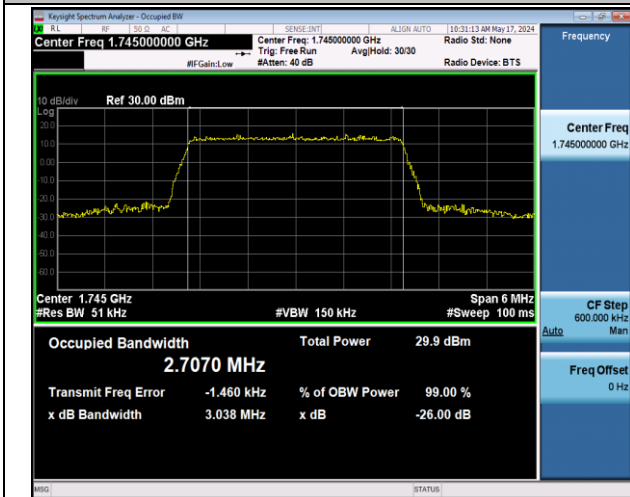
Band66-3MHz-16QAM-132322-15RB#0-PASS
