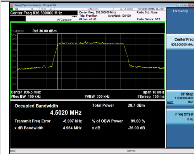
Band5-5MHz-16QAM-20525-25RB#0-PASS
