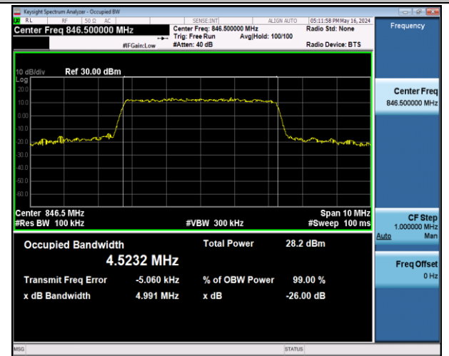
Band5-5MHz-16QAM-20625-25RB#0-PASS
