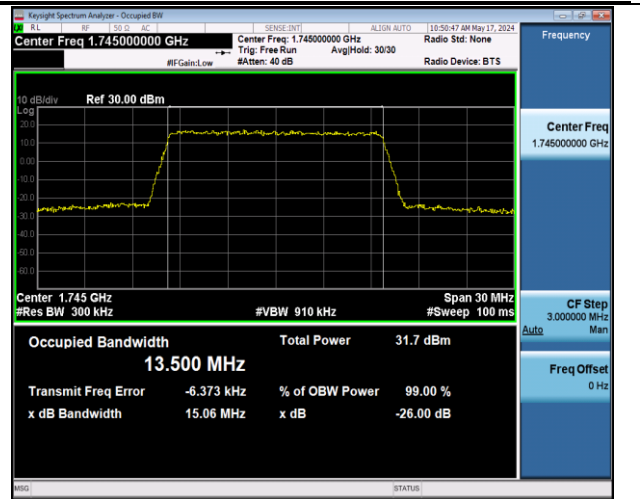
Band66-15MHz-QPSK-132322-75RB#0-PASS
