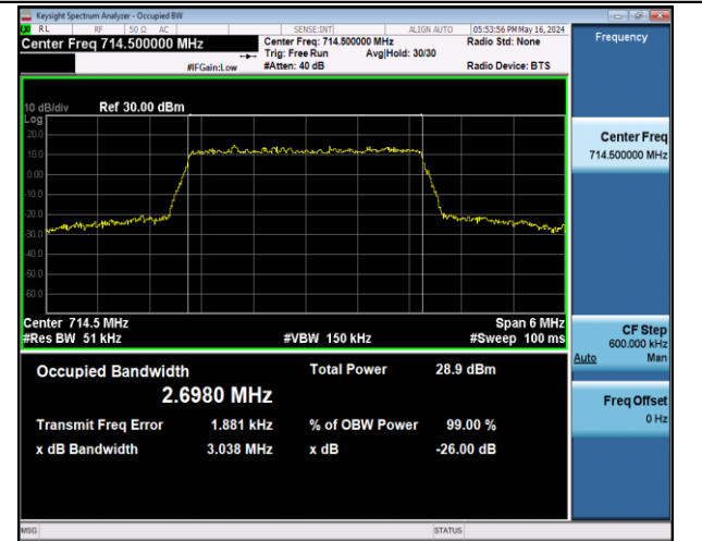
Band12-3MHz-16QAM-23165-15RB#0-PASS
