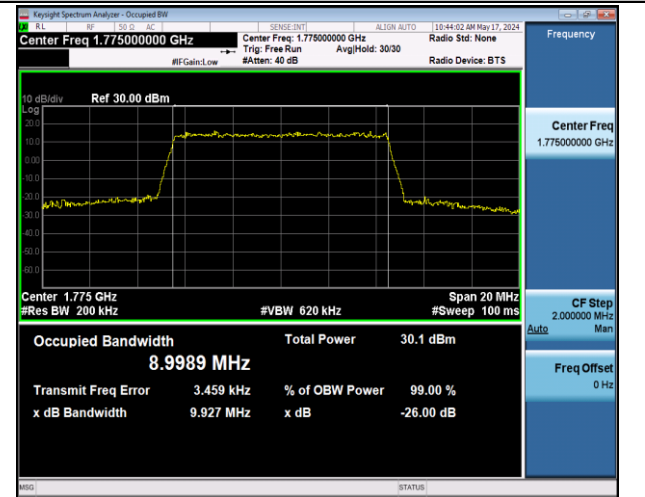
Band66-10MHz-16QAM-132622-50RB#0-PASS
