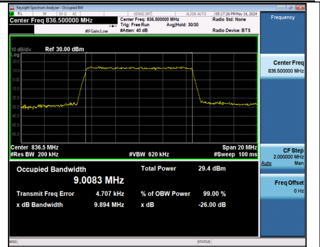
Band5-10MHz-QPSK-20525-50RB#0-PASS
