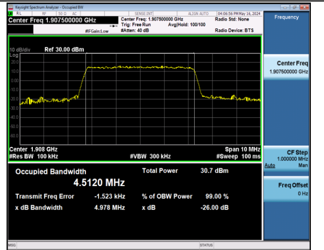
Band2-5MHz-16QAM-19175-25RB#0-PASS
