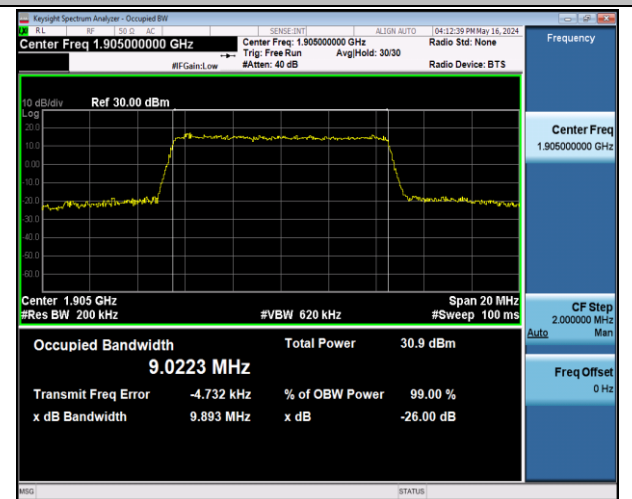
Band2-10MHz-16QAM-19150-50RB#0-PASS
