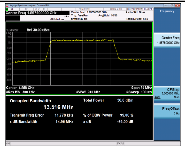
Band2-15MHz-16QAM-18675-75RB#0-PASS
