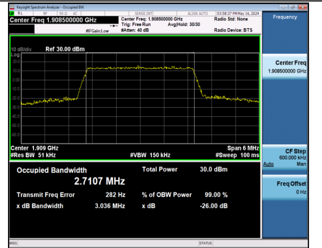
Band2-3MHz-16QAM-19185-15RB#0-PASS
