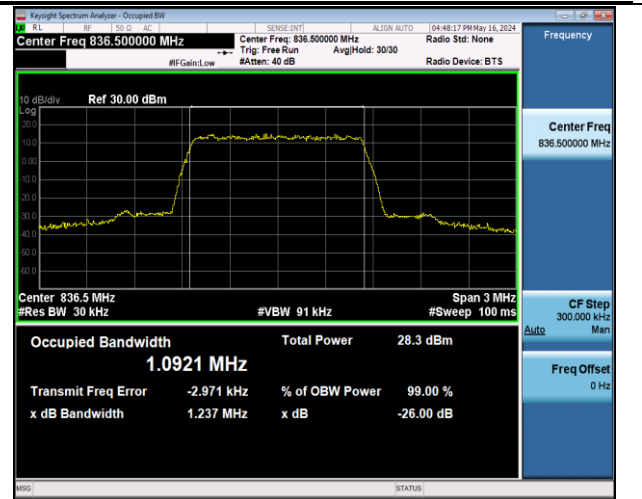
Band5-1.4MHz-QPSK-20525-6RB#0-PASS
