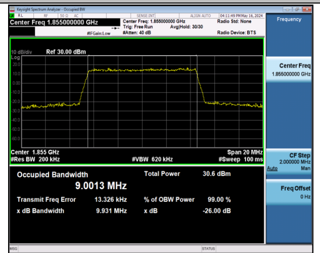
Band2-10MHz-16QAM-18650-50RB#0-PASS
