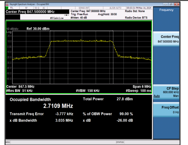
Band5-3MHz-16QAM-20635-15RB#0-PASS
