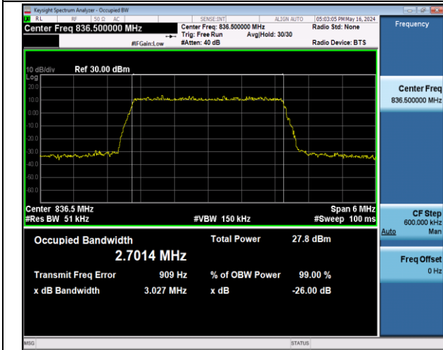
Band5-3MHz-16QAM-20525-15RB#0-PASS
