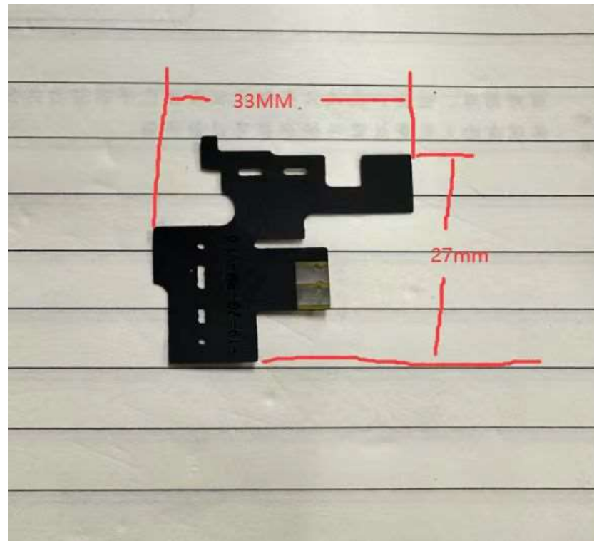
GSM ANT Wide=33mm Length=27mm
