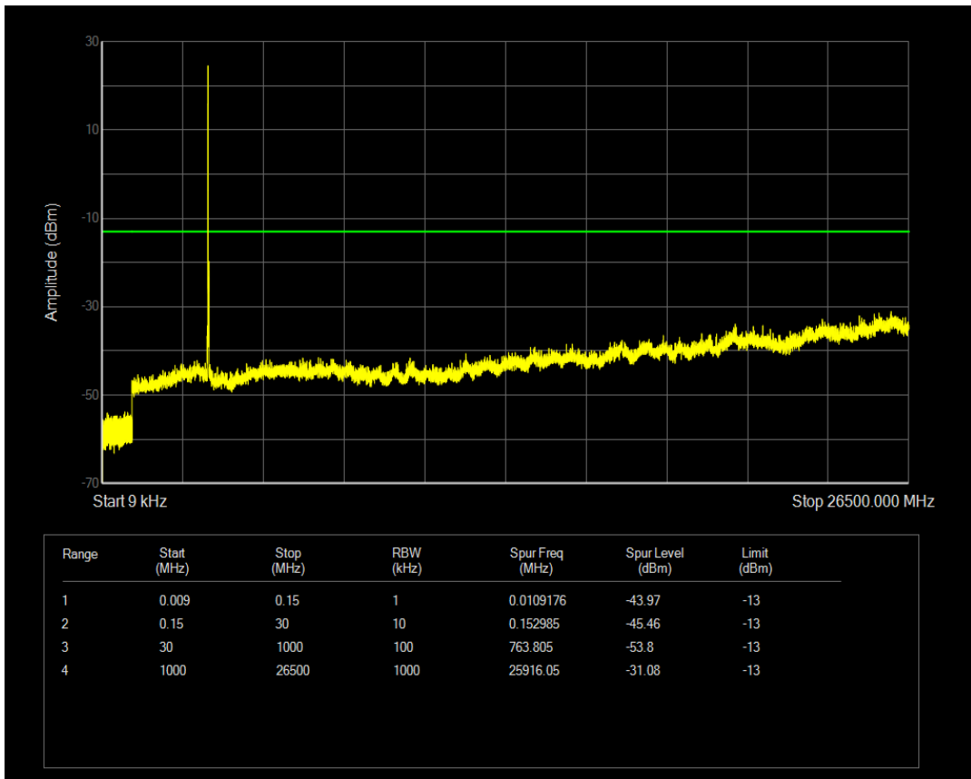
Band42 QAM16 BW=15MHz Channel=42590 RB Size=1 Position=#0
