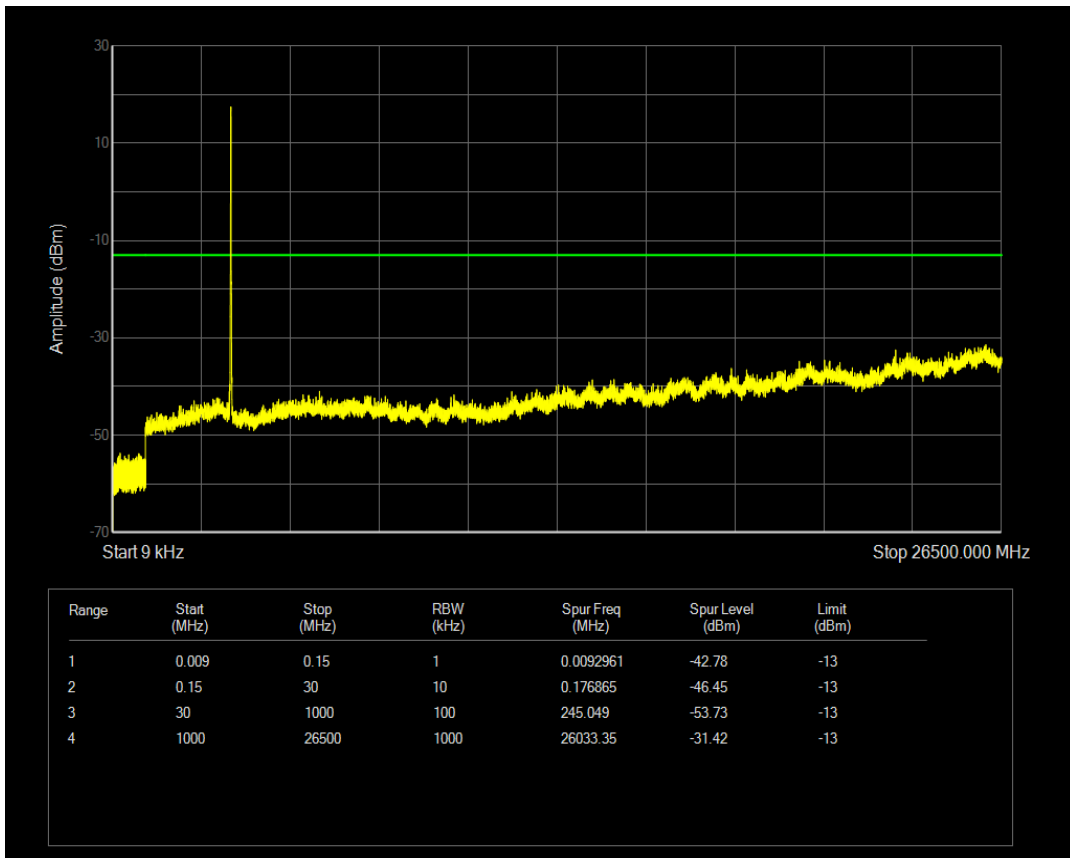
Band42 QAM16 BW=15MHz Channel=43015 RB Size=1 Position=#0
