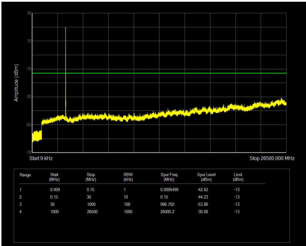
Band42 QAM16 BW=10MHz Channel=42590 RB Size=1 Position=#0
