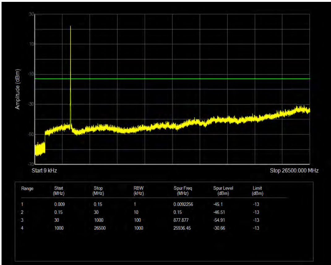
Band42 16QAM BW=10MHz Channel=42140 RB Size=1 Position=#0
