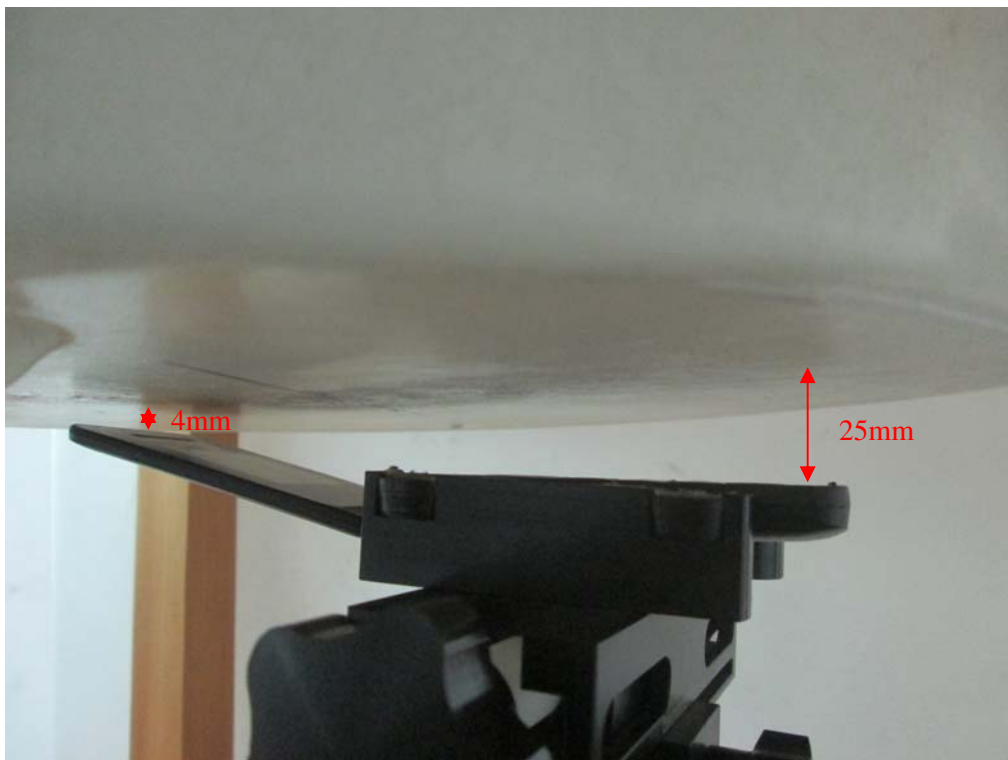
Head Check Setup Photo
