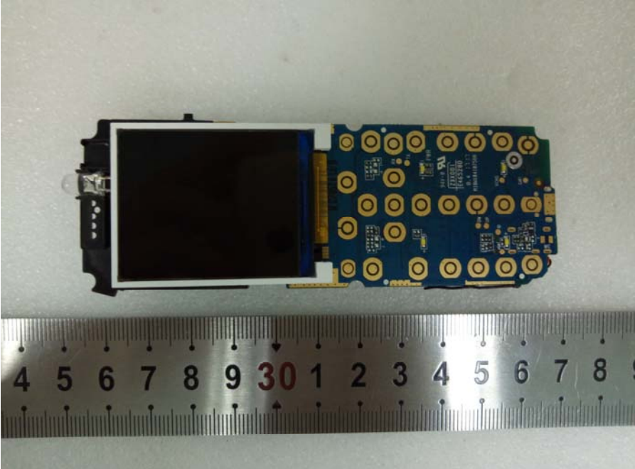
EUT – Main Board Front Shielding off View
