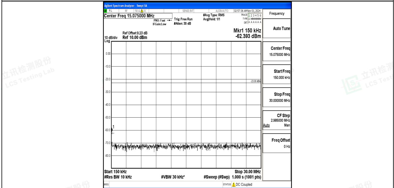
Band5-10MHz-QPSK-20450-1RB#0-0.15~30-PASS
