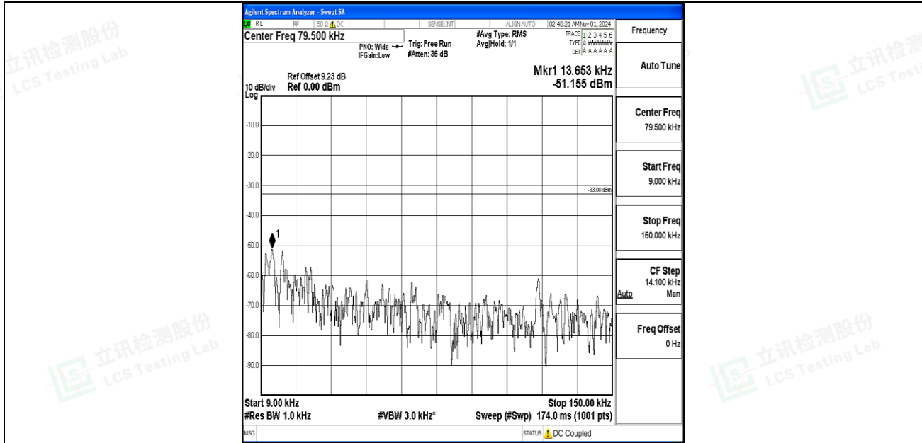
Band5-5MHz-QPSK-20525-1RB#0-0.009~0.15-PASS
