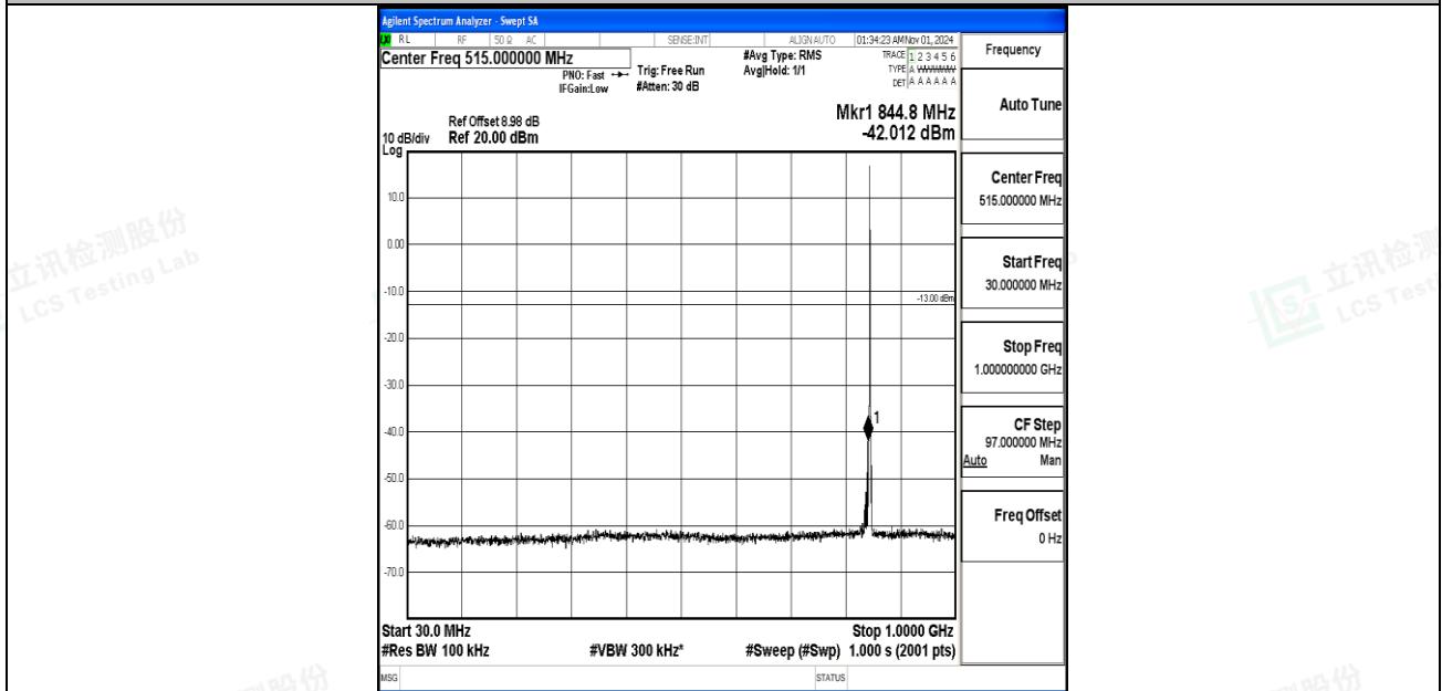
Band5-1.4MHz-16QAM-20643-1RB#0-30~1000-PASS
