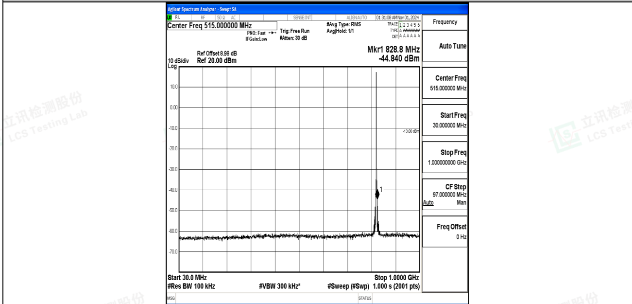
Band5-1.4MHz-16QAM-20407-1RB#0-30~1000-PASS
