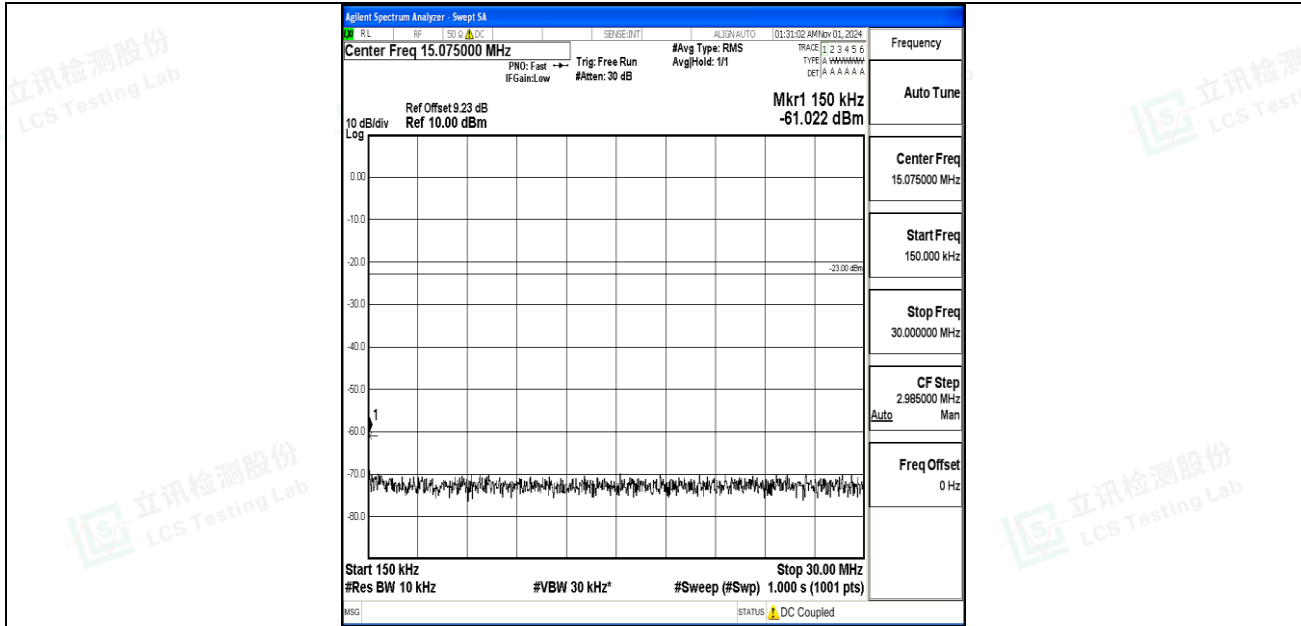
Band5-1.4MHz-16QAM-20407-1RB#0-0.15~30-PASS
