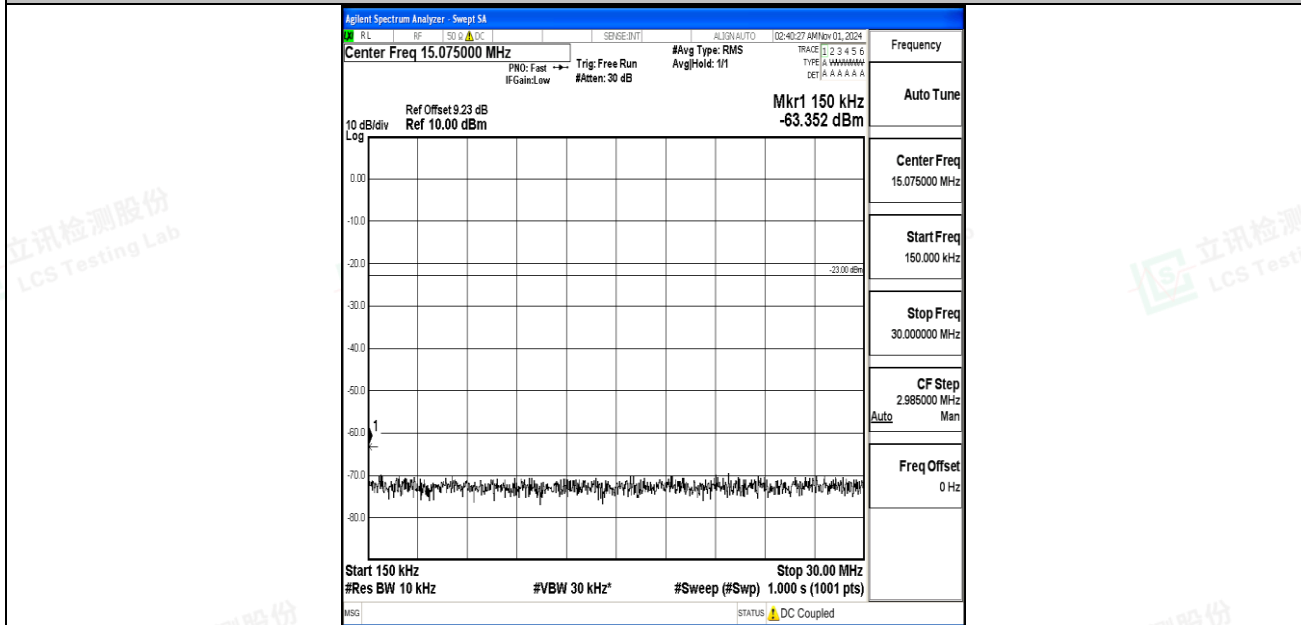
Band5-5MHz-QPSK-20525-1RB#0-0.15~30-PASS
