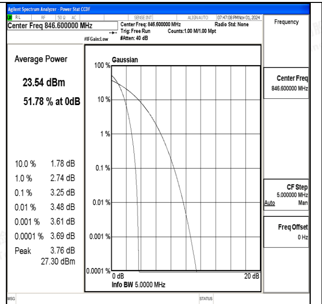
Channel 4233 / 846.6 MHz
