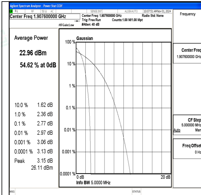
Channel 9538 / 1907.6 MHz
