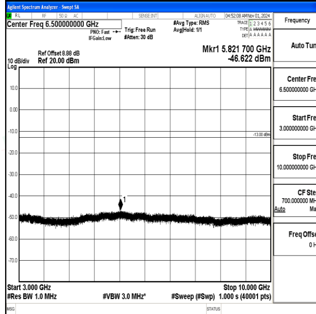
Band12-10MHz-16QAM-23060-1RB#0-3000~10000-PASS
