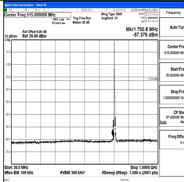
Band12-5MHz-16QAM-23155-1RB#0-30~1000-PASS
