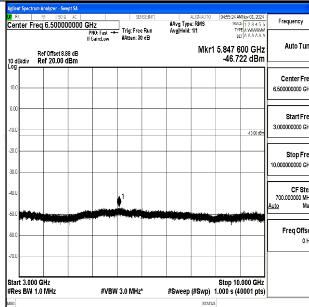
Band12-10MHz-16QAM-23130-1RB#0-3000~10000-PASS
