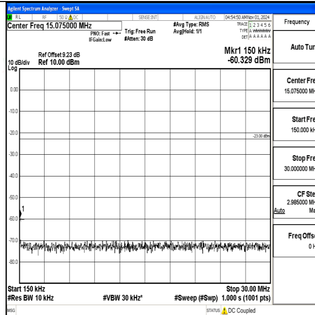
Band12-10MHz-16QAM-23130-1RB#0-0.15~30-PASS
