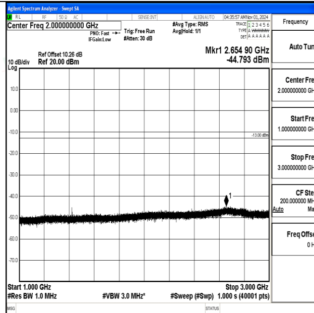
Band12-5MHz-16QAM-23155-1RB#0-1000~3000-PASS
