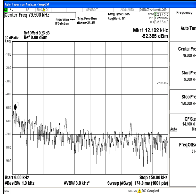
Band12-10MHz-16QAM-23060-1RB#0-0.009~0.15-PASS
