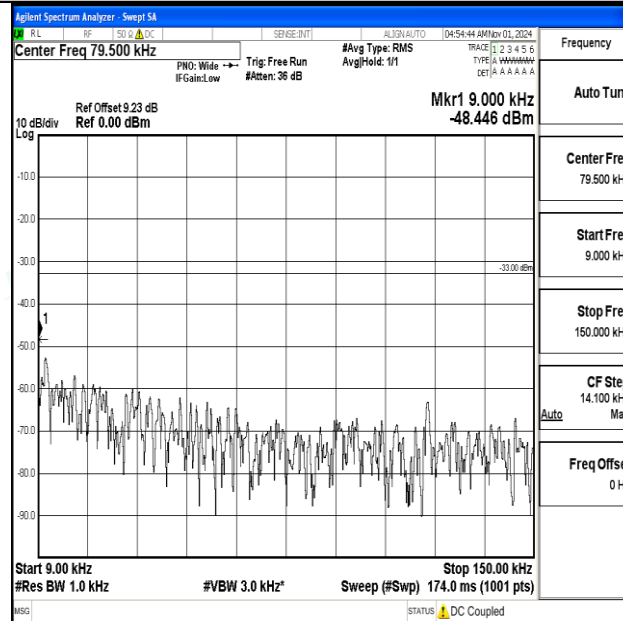
Band12-10MHz-16QAM-23130-1RB#0-0.009~0.15-PASS
