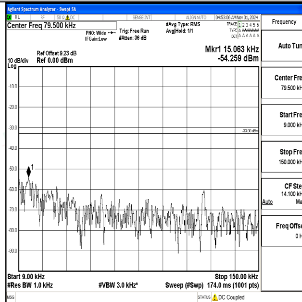
Band12-10MHz-16QAM-23095-1RB#0-0.009~0.15-PASS
