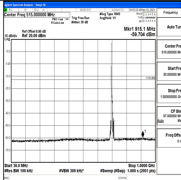
Band12-10MHz-16QAM-23095-1RB#0-30~1000-PASS
