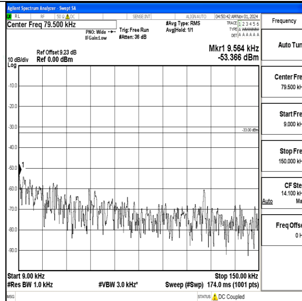
Band12-10MHz-QPSK-23060-1RB#0-0.009~0.15-PASS
