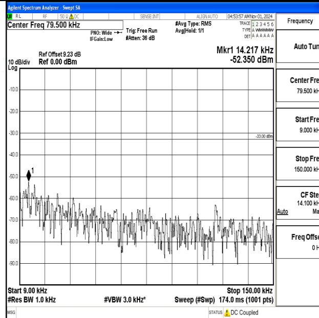
Band12-10MHz-QPSK-23130-1RB#0-0.009~0.15-PASS
