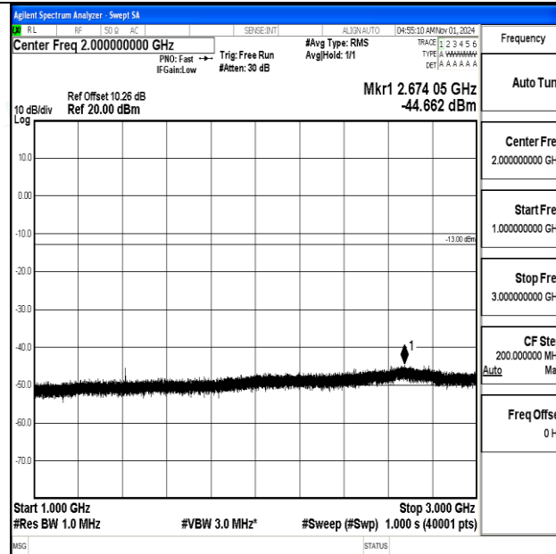
Band12-10MHz-16QAM-23130-1RB#0-1000~3000-PASS
