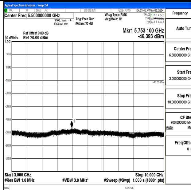
Band12-10MHz-16QAM-23095-1RB#0-3000~10000-PASS
