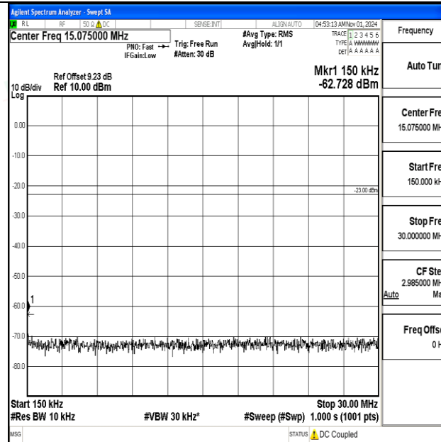
Band12-10MHz-16QAM-23095-1RB#0-0.15~30-PASS
