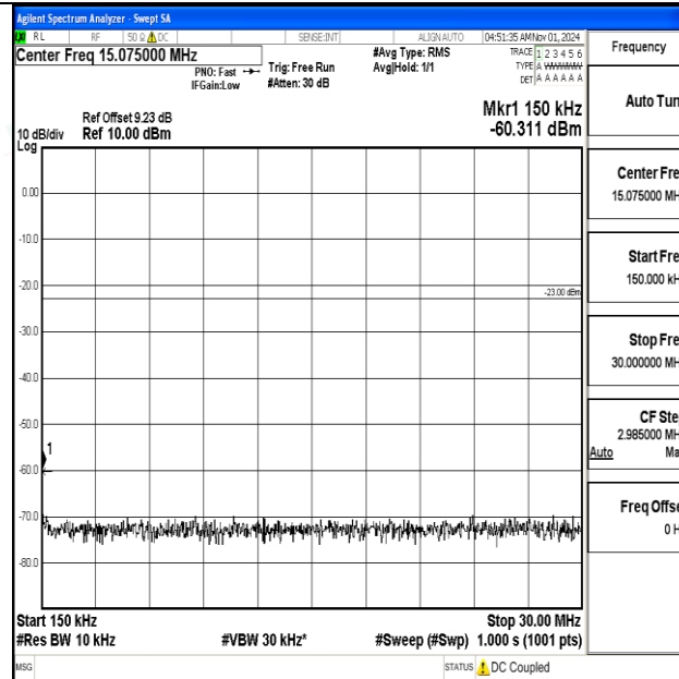
Band12-10MHz-16QAM-23060-1RB#0-0.15~30-PASS
