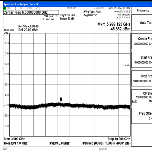
Band12-5MHz-16QAM-23155-1RB#0-3000~10000-PASS
