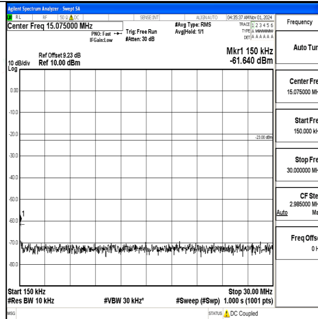
Band12-5MHz-16QAM-23155-1RB#0-0.15~30-PASS
