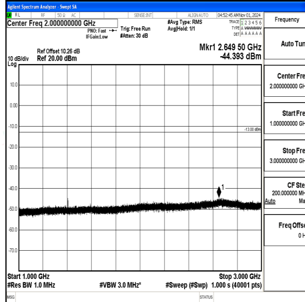
Band12-10MHz-QPSK-23095-1RB#0-1000~3000-PASS
