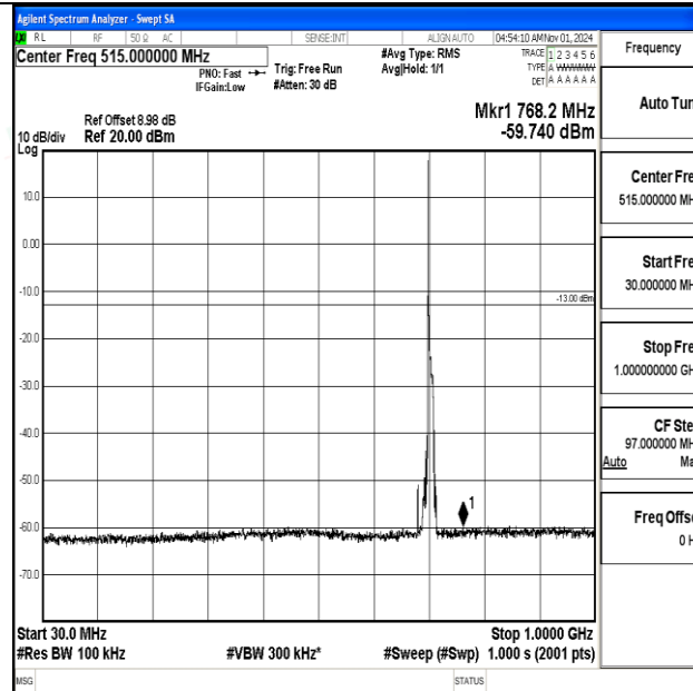
Band12-10MHz-QPSK-23130-1RB#0-30~1000-PASS
