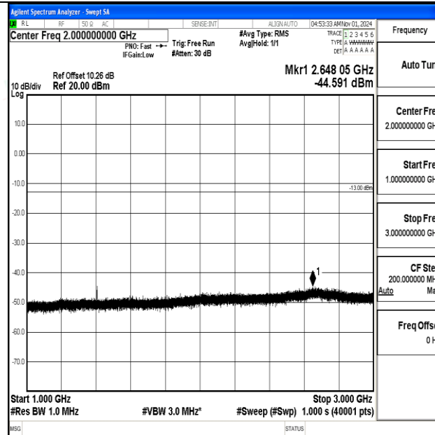
Band12-10MHz-16QAM-23095-1RB#0-1000~3000-PASS
