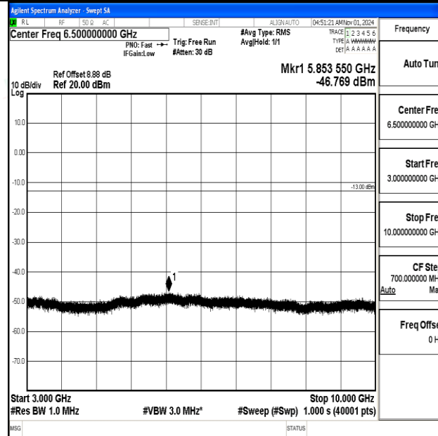
Band12-10MHz-QPSK-23060-1RB#0-3000~10000-PASS
