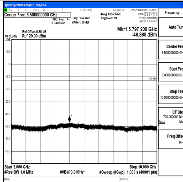
Band12-10MHz-QPSK-23095-1RB#0-3000~10000-PASS
