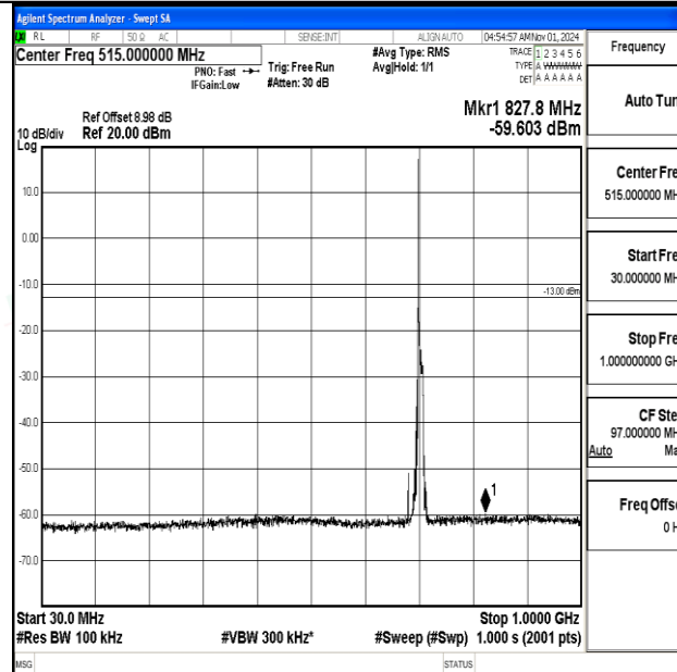
Band12-10MHz-16QAM-23130-1RB#0-30~1000-PASS
