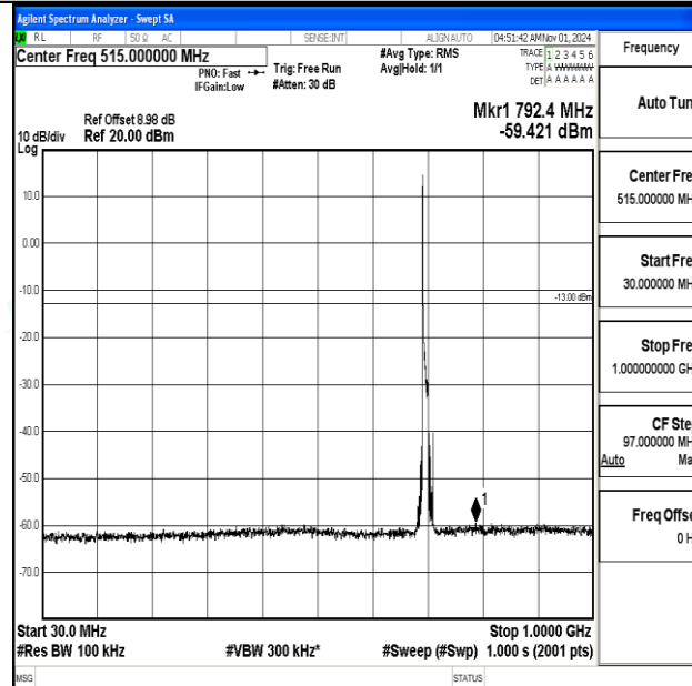
Band12-10MHz-16QAM-23060-1RB#0-30~1000-PASS
