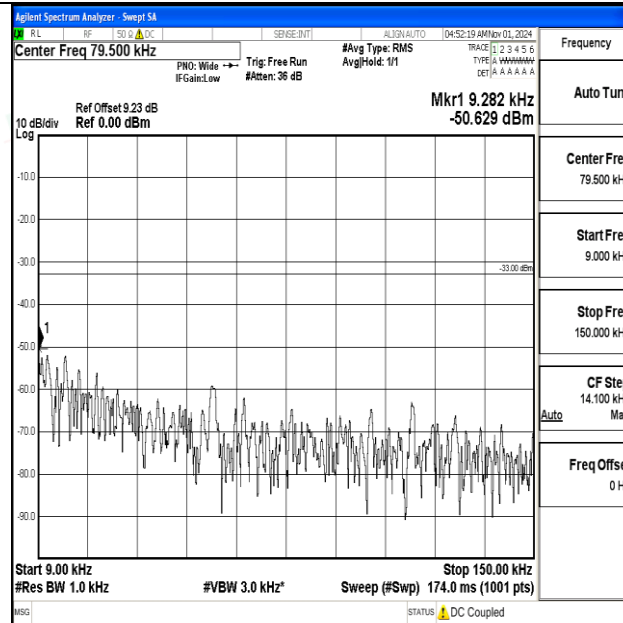
Band12-10MHz-QPSK-23095-1RB#0-0.009~0.15-PASS
