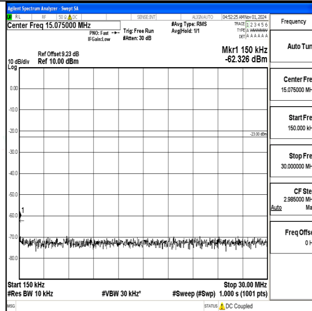
Band12-10MHz-QPSK-23095-1RB#0-0.15~30-PASS
