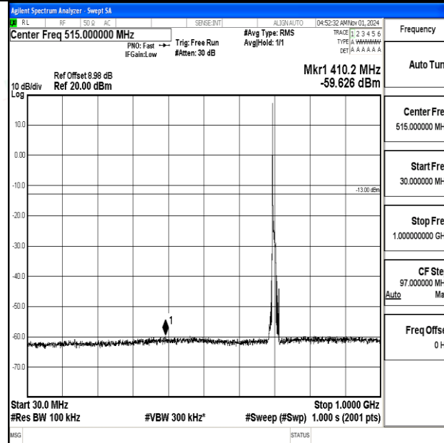
Band12-10MHz-QPSK-23095-1RB#0-30~1000-PASS
