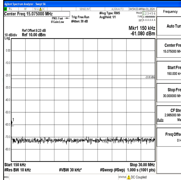
Band12-10MHz-QPSK-23130-1RB#0-0.15~30-PASS
