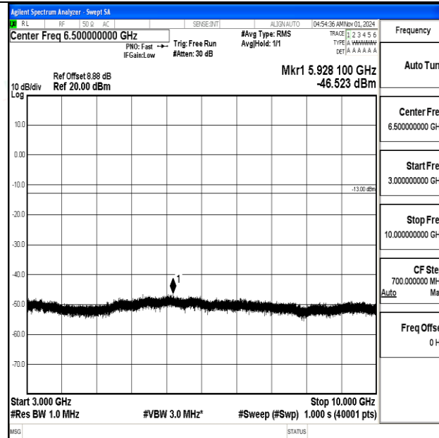
Band12-10MHz-QPSK-23130-1RB#0-3000~10000-PASS
