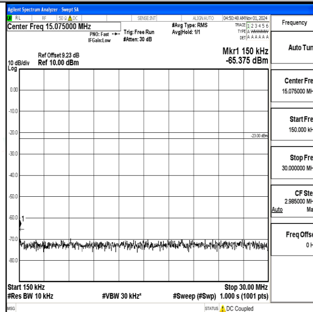
Band12-10MHz-QPSK-23060-1RB#0-0.15~30-PASS
