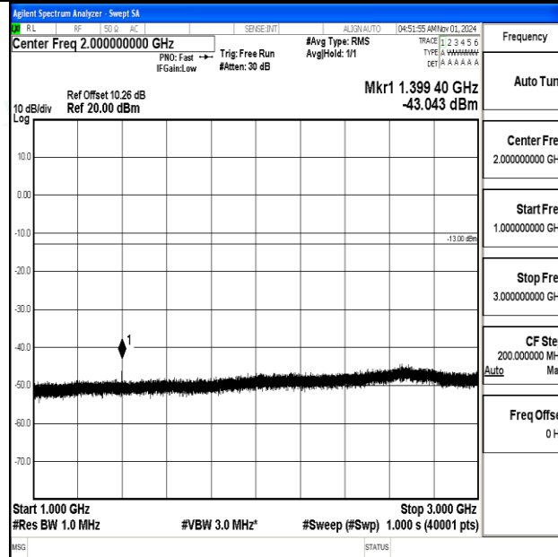
Band12-10MHz-16QAM-23060-1RB#0-1000~3000-PASS
