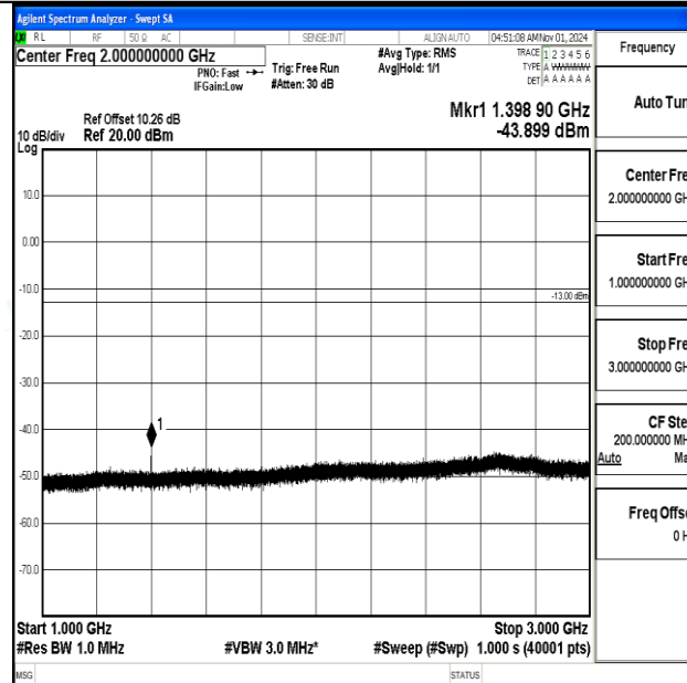
Band12-10MHz-QPSK-23060-1RB#0-1000~3000-PASS
