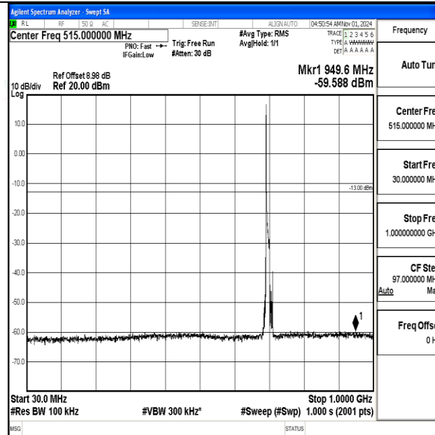
Band12-10MHz-QPSK-23060-1RB#0-30~1000-PASS
