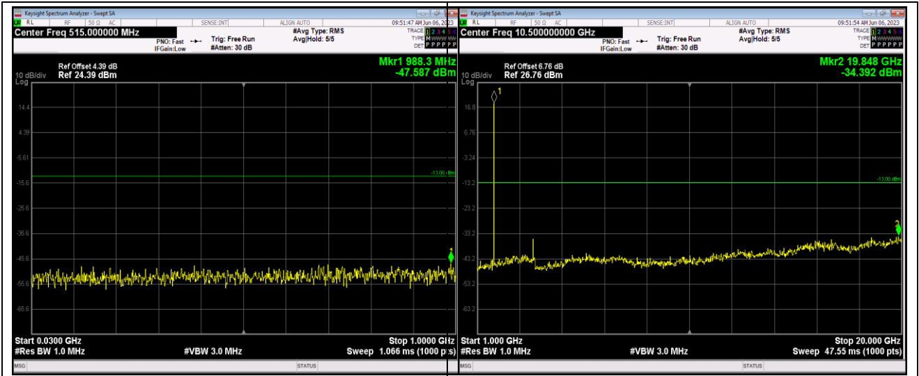
Band4-20MHz-QPSK-20050-1RB#0-Range1:30~1000MHz
