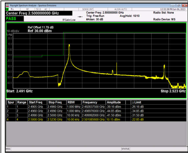
Band7-20MHz-QPSK-20850-100RB#0
