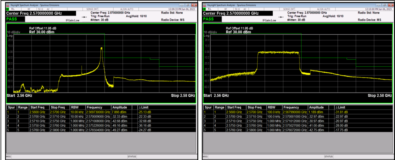
Band7-5MHz-16QAM-20775-1RB#0
