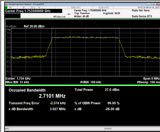
Band4-3MHz-16QAM-20175-15RB#0
