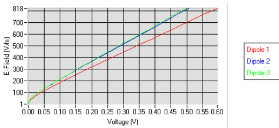
Calibration curves
