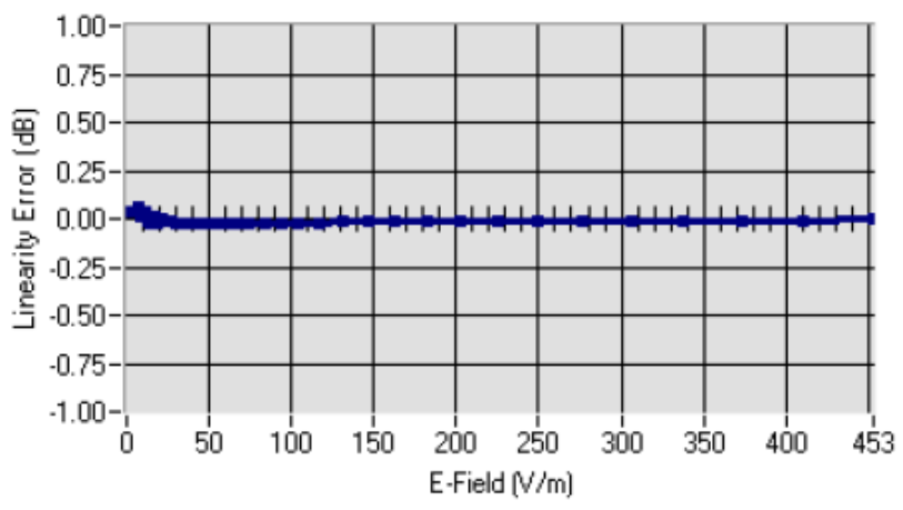
Linearity
