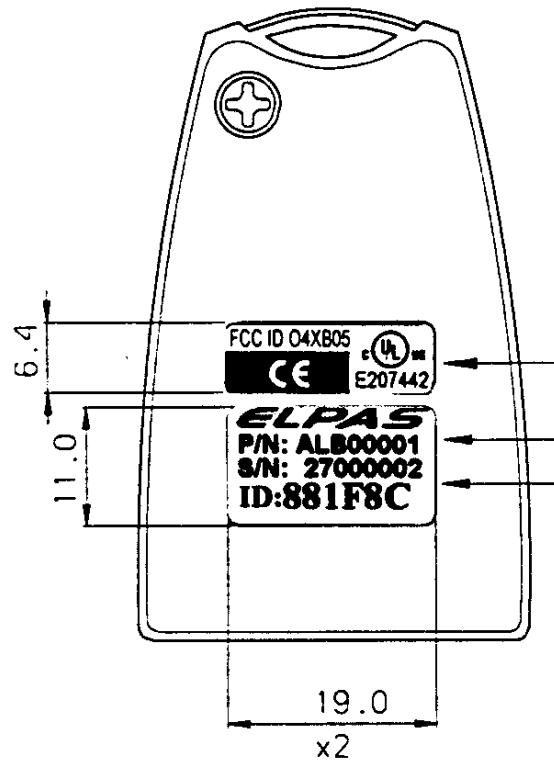
Figure 1. FCC Label
