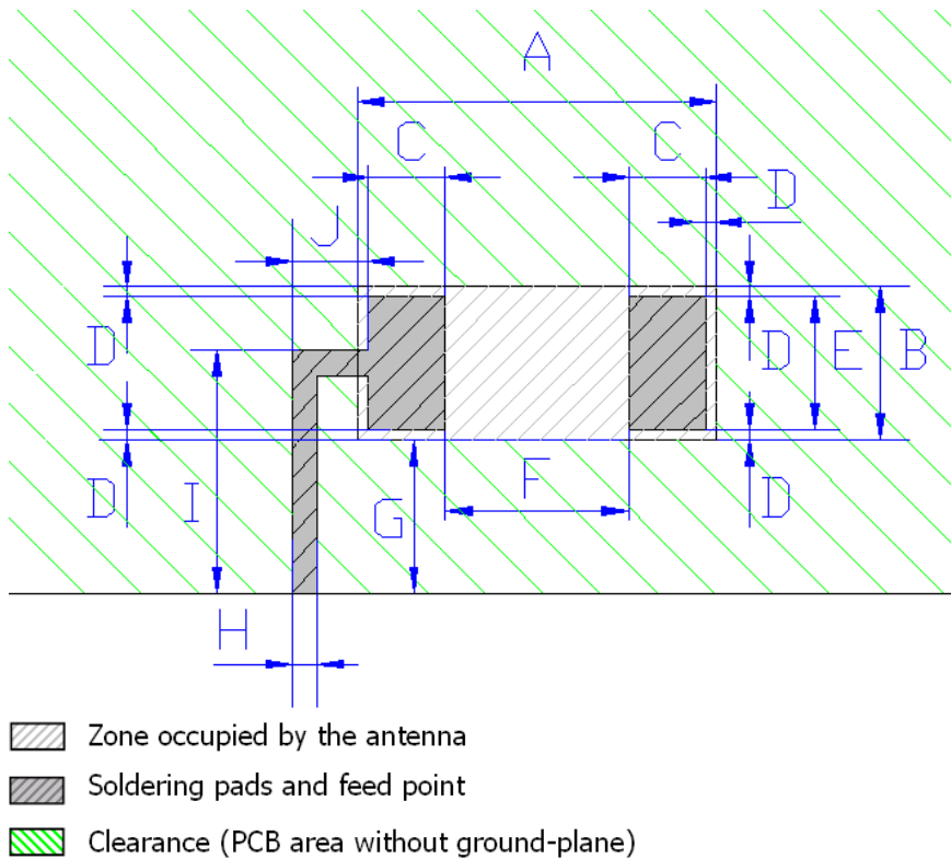
Figure 3 – Antenna Footprint Details
