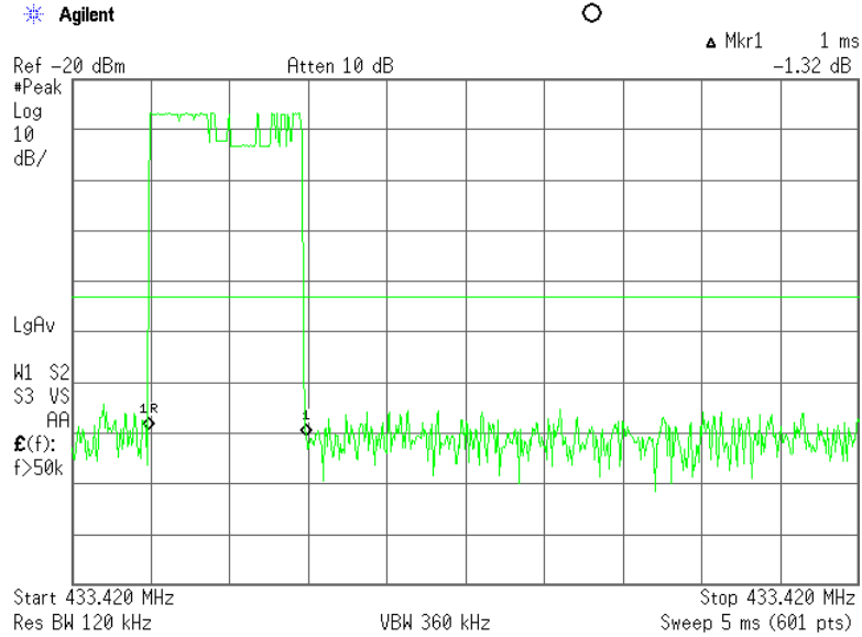
Plot 7.1.5 Polling / supervision transmission duration
