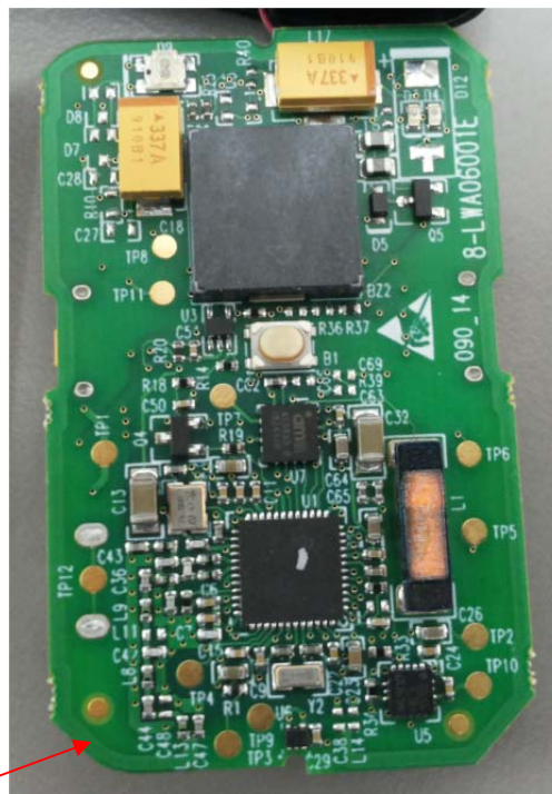
Photograph 7.4.1 Antenna assembly
