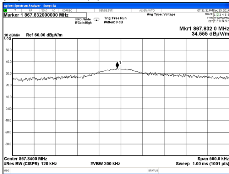
Plot 7.2.13 Radiated emission measurements at the second harmonic frequency
