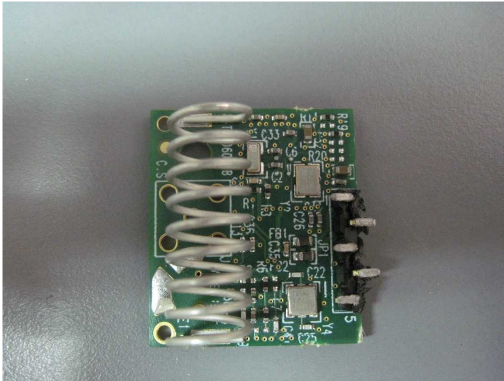
433 MHz transmitter
