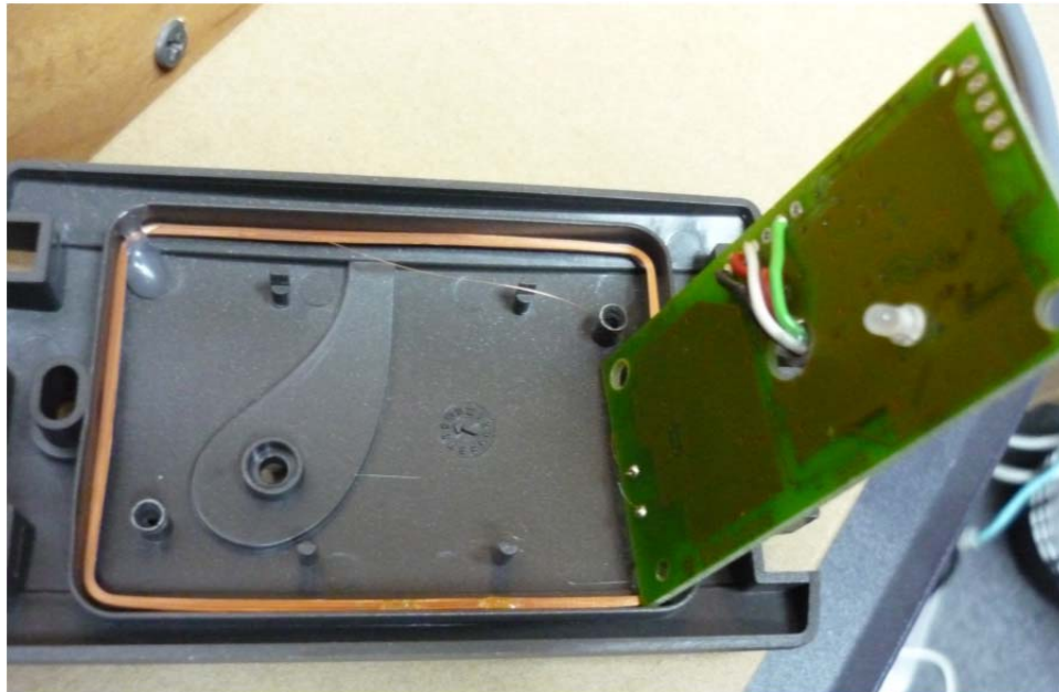
Photograph 7.3.1 Antenna assembly
