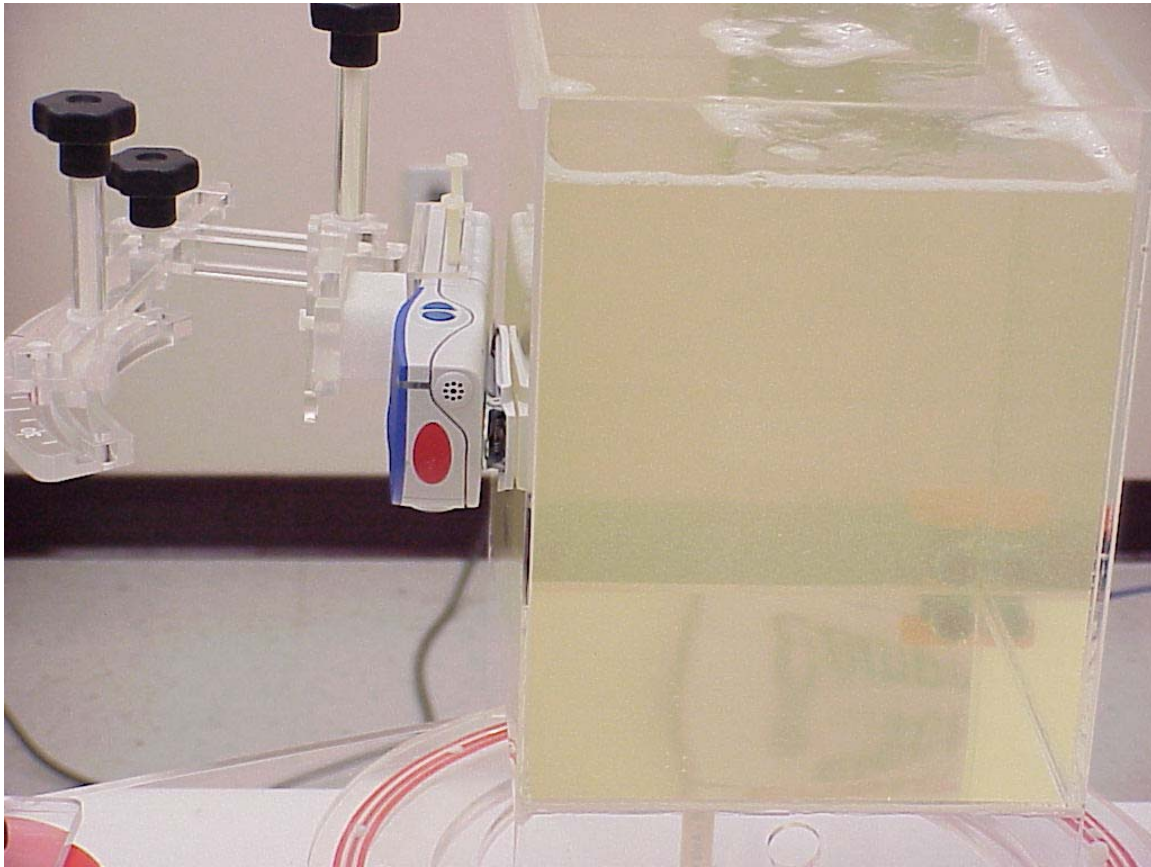
Photo 7. Body SAR
