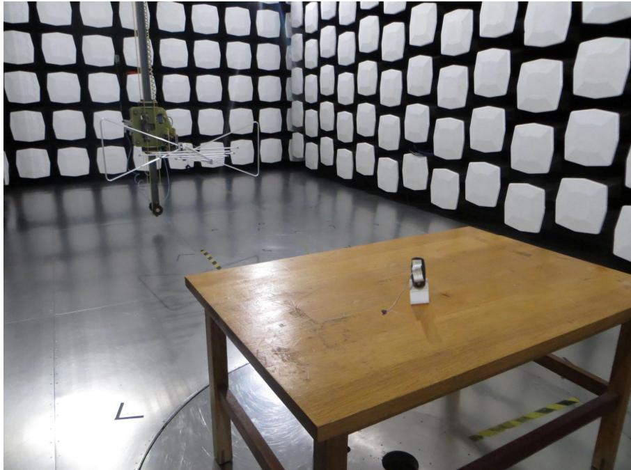
Below 1GHz
