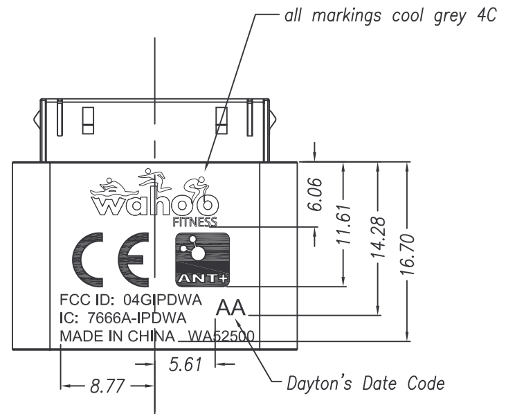
bottom case w/markings A1-4136003
