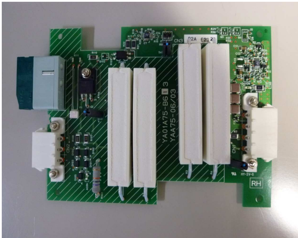
top view
