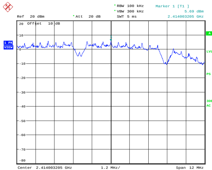
Figure 42: Power Spectral Density, Antenna 2, Mode A (2412MHz)
