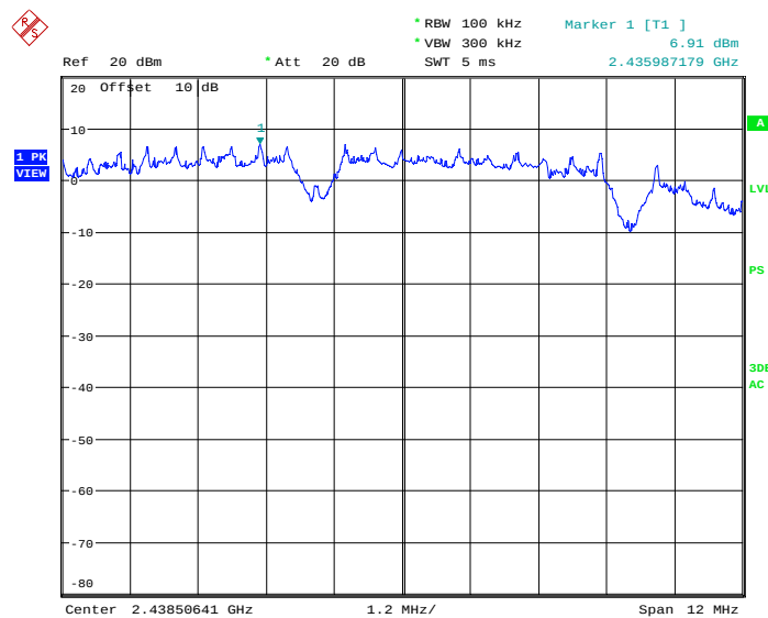
Figure 40: Power Spectral Density, Antenna 1, Mode B (2437MHz)
