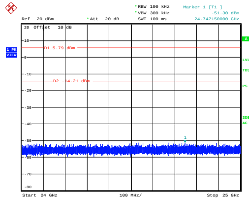
Figure 26: Conducted Spurious Emissions, 24 - 25GHz, Antenna 1, Mode B (2437MHz)
