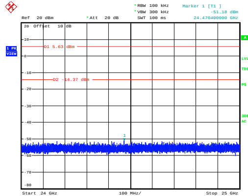
Figure 29: Conducted Spurious Emissions, 24 - 25GHz, Antenna 1, Mode C (2462MHz)
