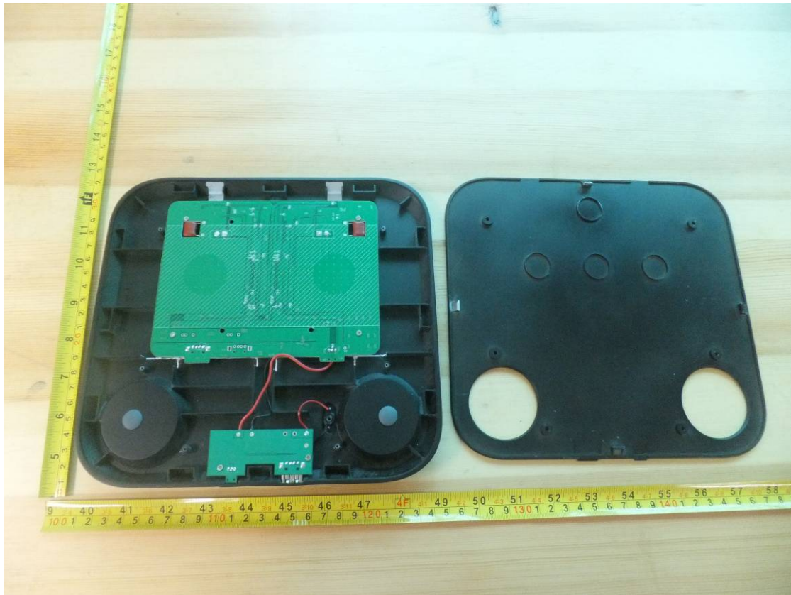
(1) EUT Photo
