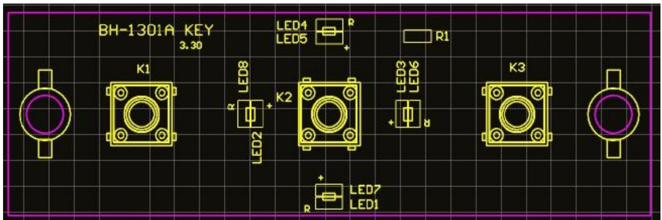
BH-1301A Key Top Overlay
