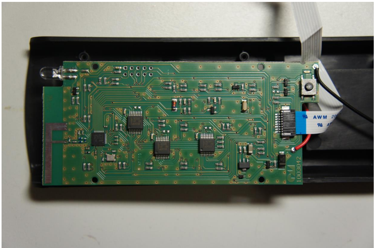
Picture 4: EUT - PCB, top side
