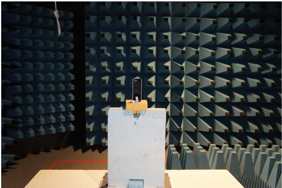
Picture 10: test setup radiated emissions > 1GHz - zoomed
