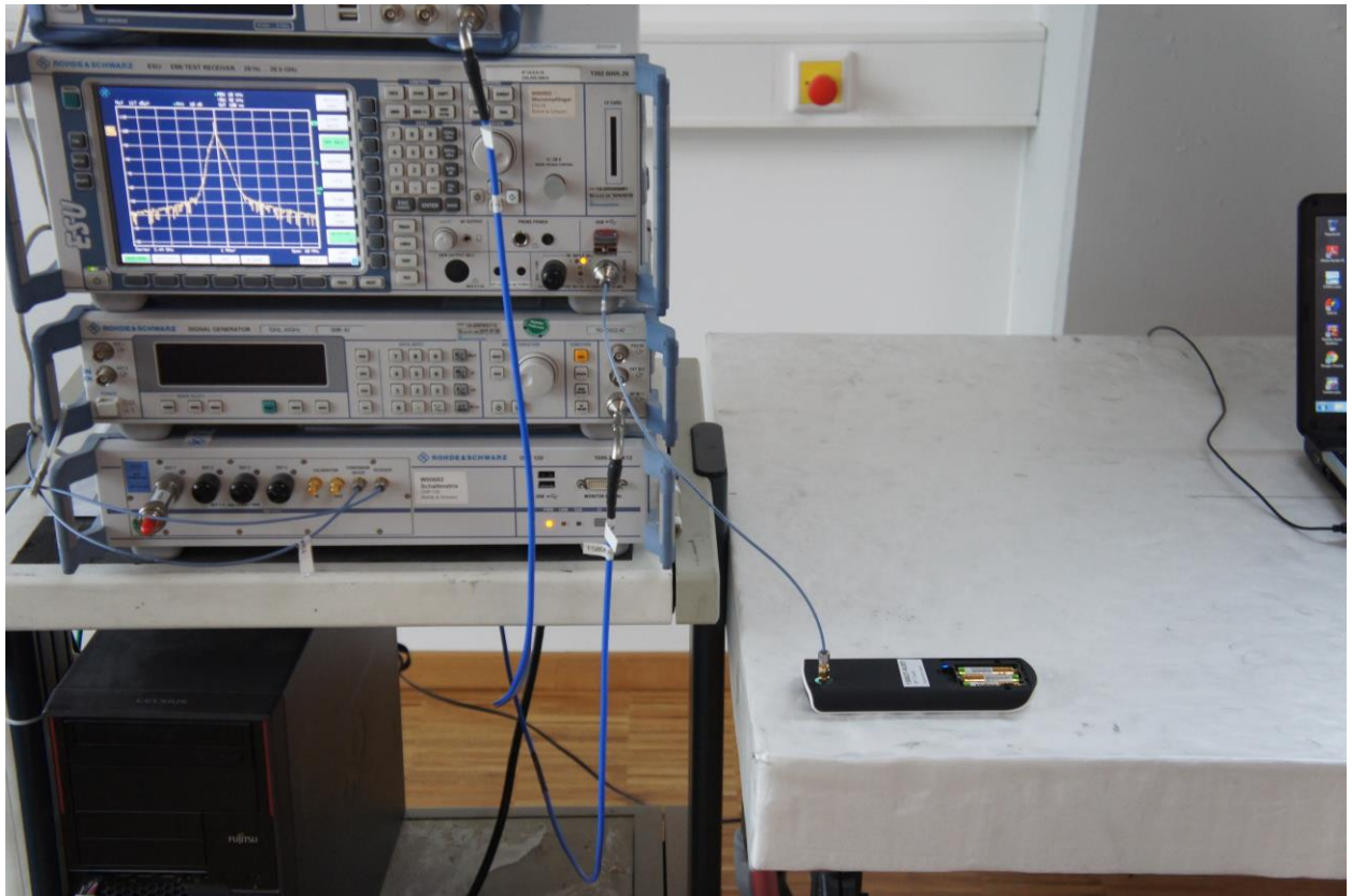
Picture 8: test setup conducted measurements
