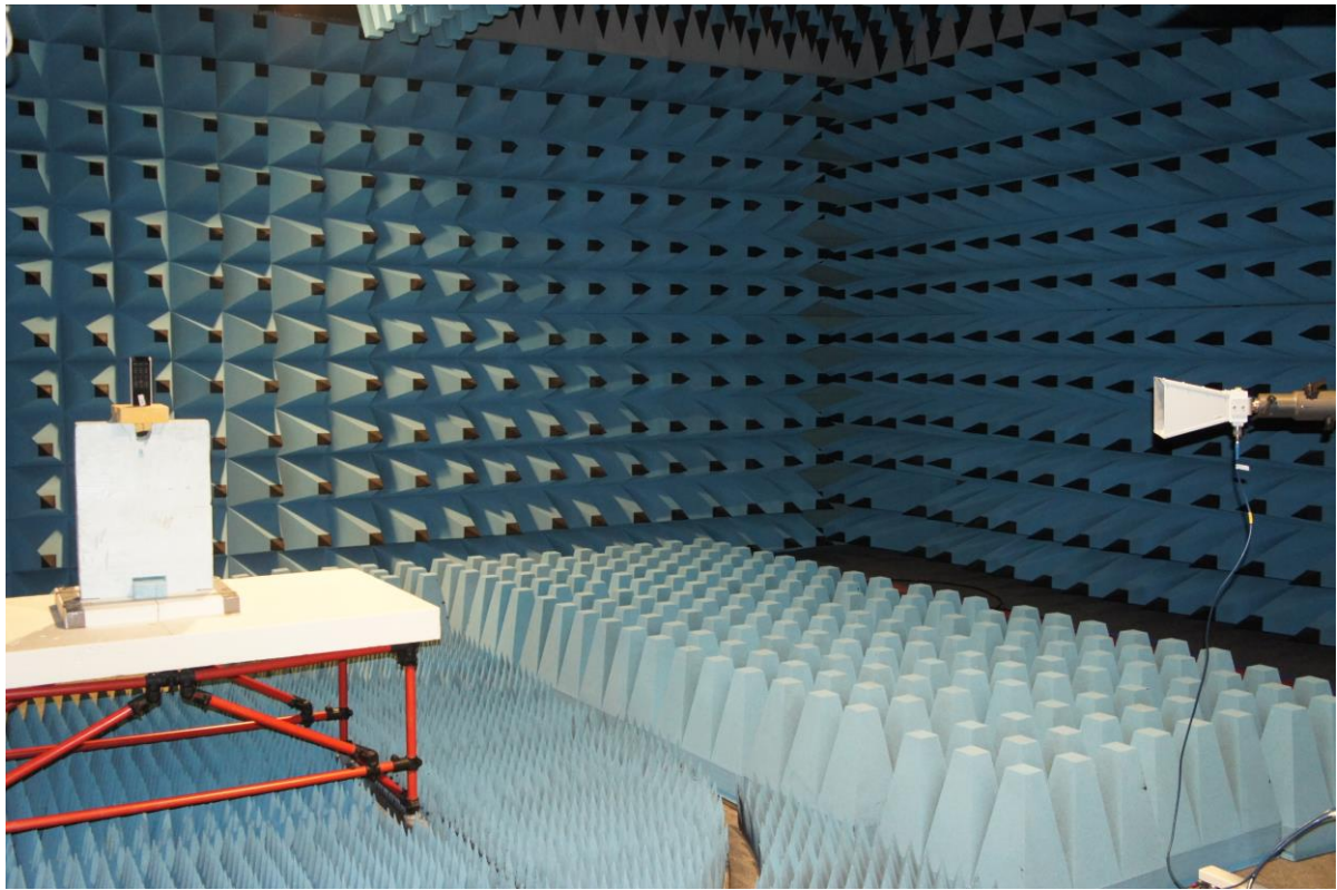
Picture 9: test setup radiated emissions > 1GHz
