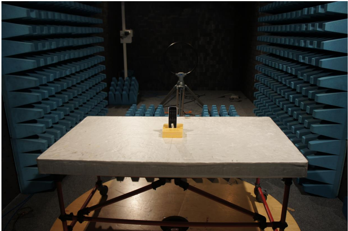
Picture 4: test setup radiated emission test 9 kHz - 30 MHz, premeasurements
