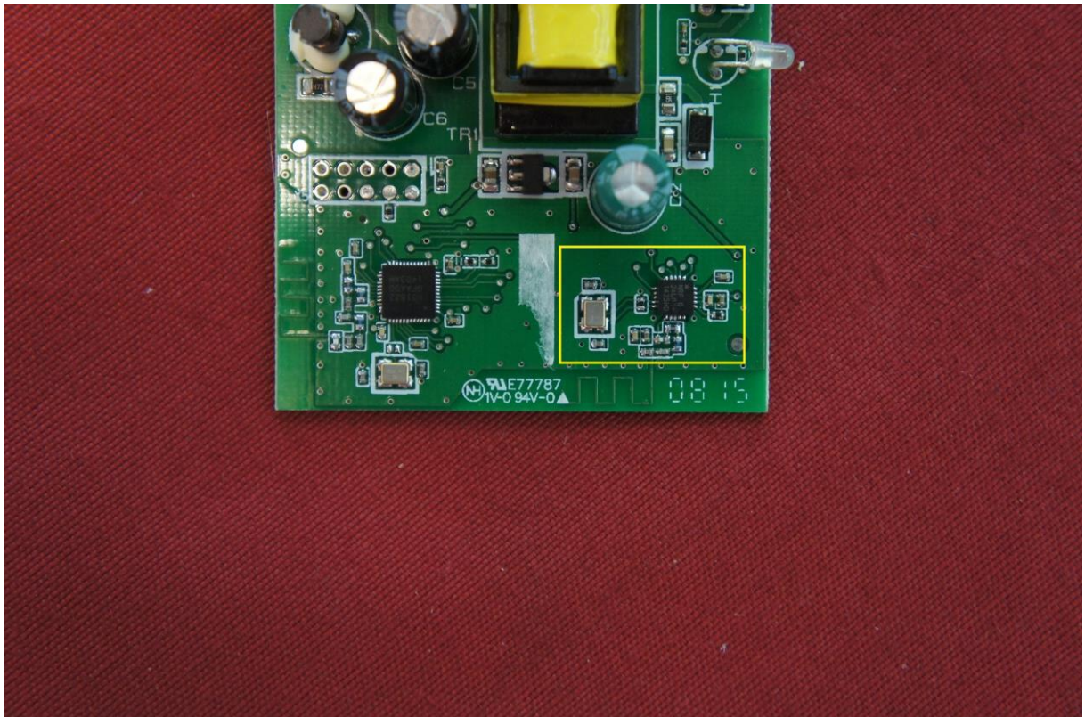
Picture 4: EUT - PCB, top side zoomed to RF part
