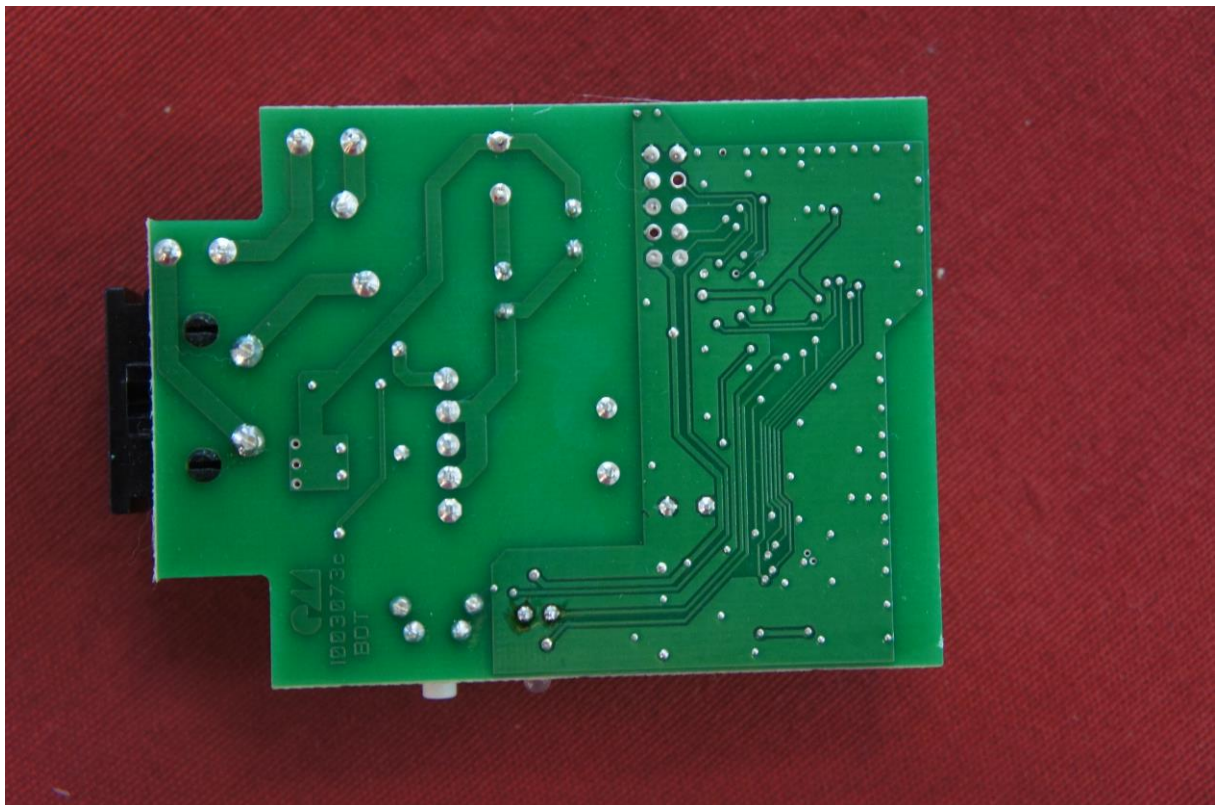
Picture 2: EUT - PCB, bottom side
