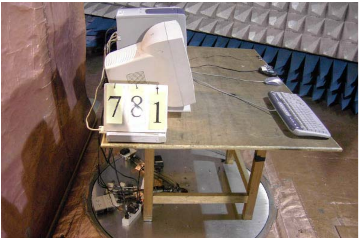
Side View of the Test Configuration
