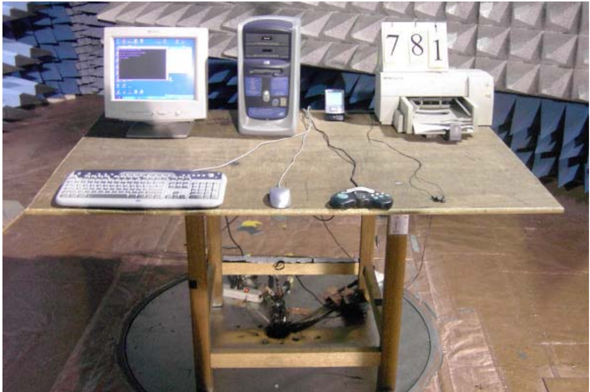
Front View of the Test Configuration of Unintentional
