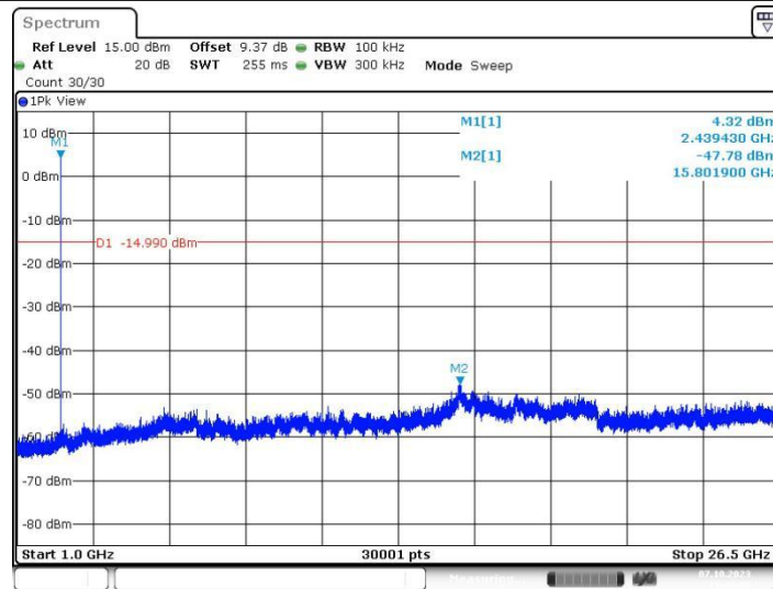
BLE_1M_Ant1_2440_1000~26500
