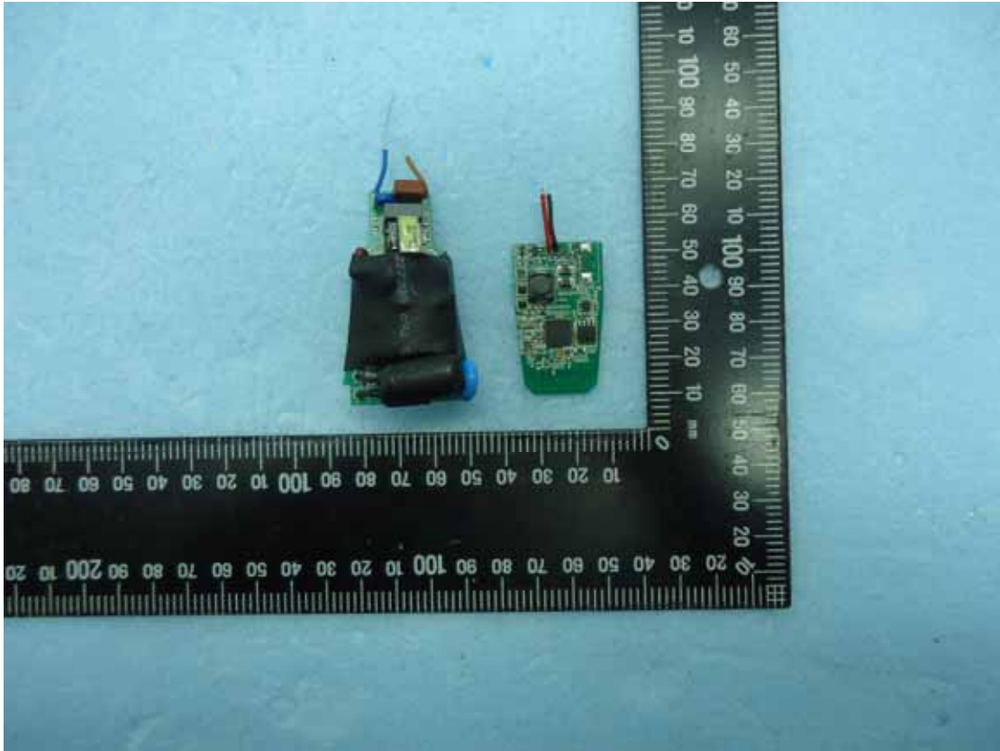
Figure 3 Internal View
