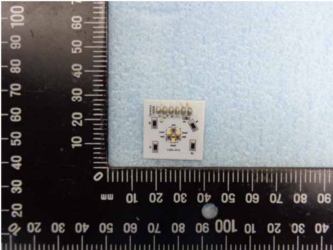
Figure 8 LED Board
