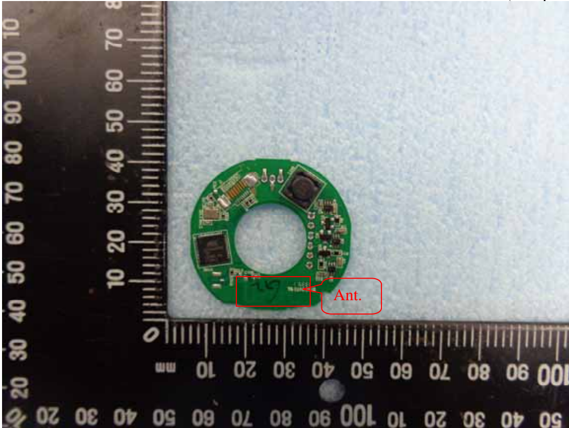
Figure 5 Wireless Board (Component Side)
