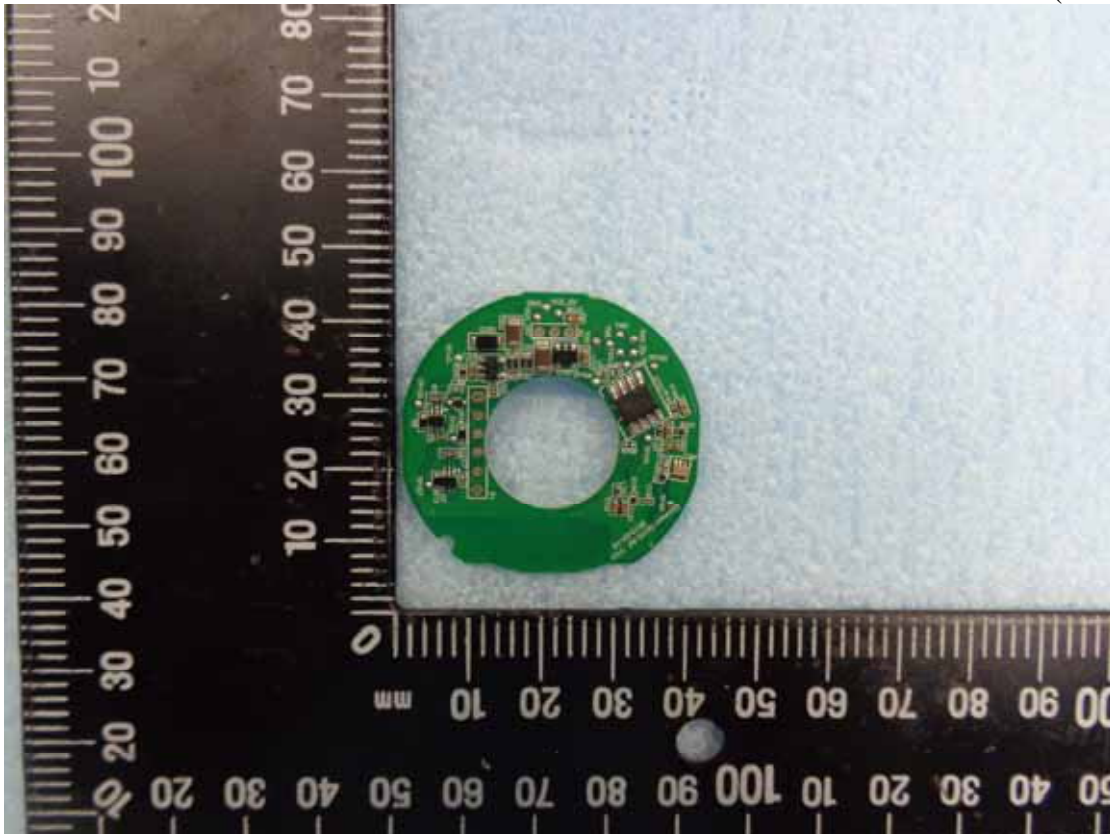
Figure 6 Wireless Board (Solder Side)
