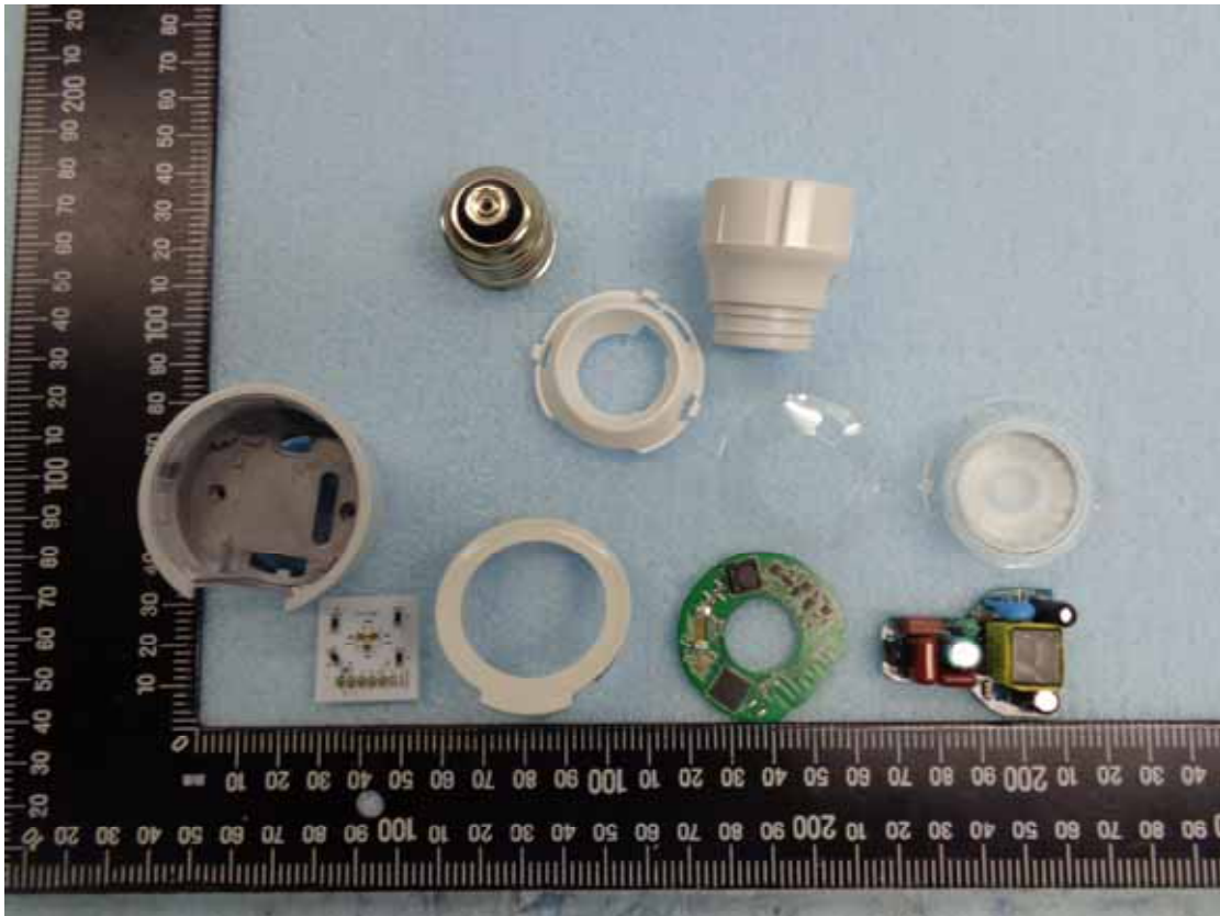
Figure 2 Internal View
