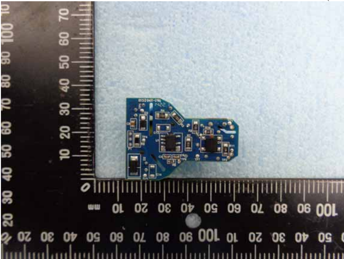
Figure 4 Power Board (Solder Side)
